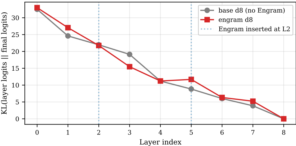
Figure A1: LogitLens — Engram converges faster in early layers
