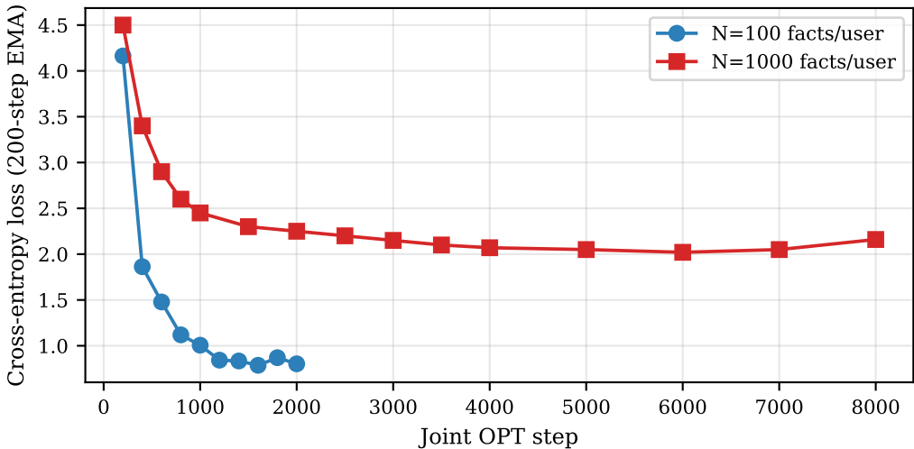
Figure A7: Joint OPT convergence on Mini-Engram-d12.
