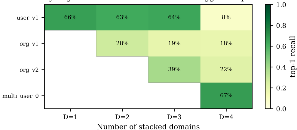
Figure A5: Multi-domain composition (top-1 per domain). Heavy degradation when domains share trigger templates.
