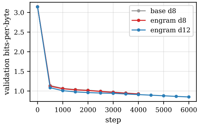
(b) Validation bpb
