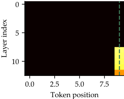
(a) Engram surgical insertion
