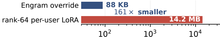
(b) Fact lifecycle avoids adapter retraining
