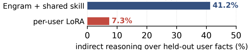
(c) Local facts support indirect and multi-hop use
