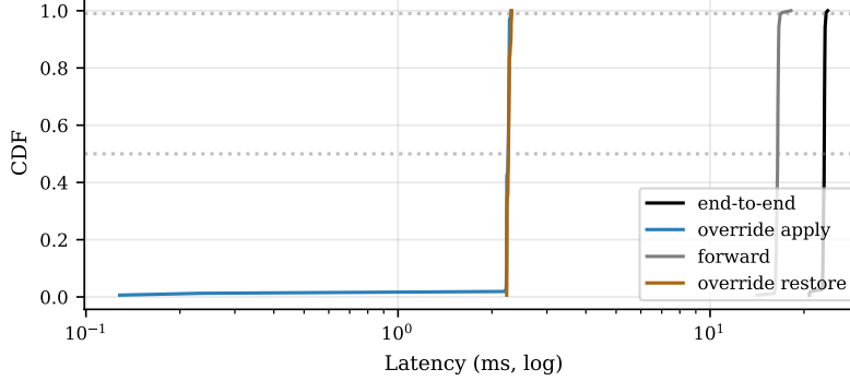
Figure 12: Per-request latency CDF on Mini-Engram-d12 (30 users \times 50 facts \times 600 requests). Override apply (blue) and restore (orange) are both sub-3 ms at p99; the forward pass (grey) dominates total latency (black).
