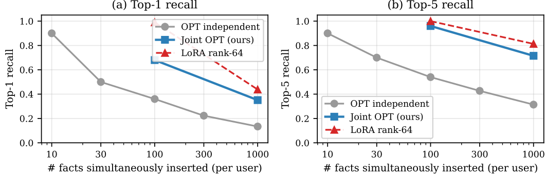
Figure 4: Within-user fact-density: top-1 (left) and top-5 (right) recall vs. number of facts inserted simultaneously into one user’s override map. Joint OPT (blue) closes most of the gap to LoRA rank-64 (red dashed) at 137× less storage.
