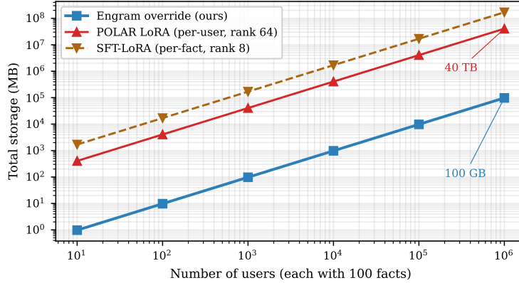
Figure 5: Storage scales linearly with user count for both approaches; Engram override is 200–1700× smaller per fact. At 1 M users × 100 facts/user, Engram storage is 100 GB vs. POLAR LoRA’s 40 TB.
