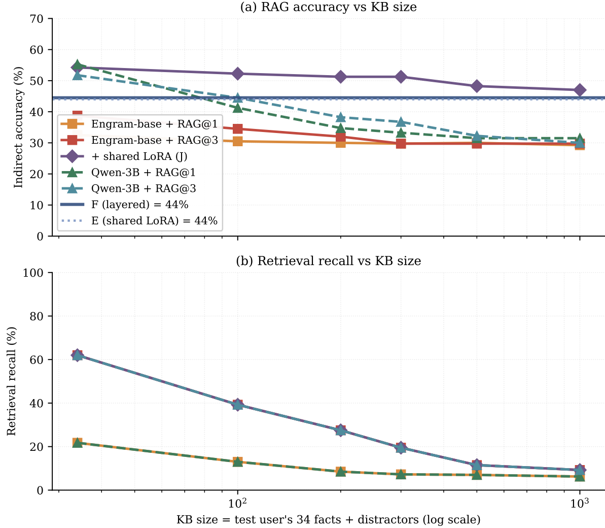
Figure 16. Indirect-reasoning accuracy and retrieval recall vs. KB size ( n=20 users, 20 indirect probes each; KB = test user’s 34 facts + distractors sampled from the 30-user schema-family pool, log x -axis, N \in \{34, 100, 200, 300, 500, 1000\} ). (a) F (layered, horizontal solid line at 44%) is invariant to KB size; the retrieval-based conditions degrade monotonically. Naive RAG and Qwen-3B + RAG fall below F at KB \geq 100 ; at KB=1000 the gap is 14 pp. J (RAG top-3 + shared LoRA) is the most robust to KB growth (54% \rightarrow 47%) because the shared reasoning skill compensates when retrieval misses, though its lead over F shrinks from 10 pp to 3 pp across the sweep. (b) Retrieval recall (fraction of probes where the retrieved set covers every fact the question needs) drops by 7\times for top-3 (62% \rightarrow 9%) between KB=34 and KB=1000, which is the mechanistic driver of (a).
