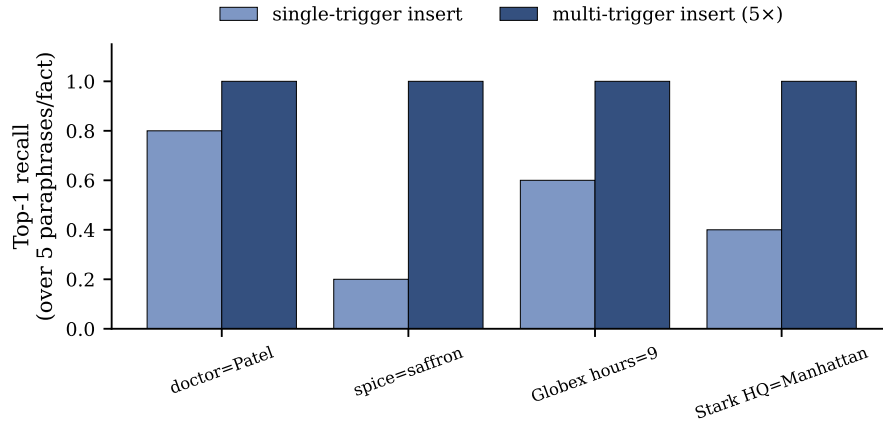
Figure 24. Paraphrase generalisation across 4 facts \times 5 paraphrases each. Single-trigger insertion gets 50% top-1 for free (suffix N-gram overlap); multi-trigger insertion (insert at all 5 paraphrases) gets 100% at 5 \times the per-fact OPT cost.
