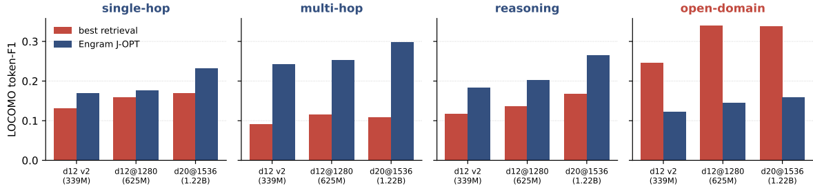
Figure 18. Locomo category breakdown (token-F1), Engram Joint OPT (blue) vs. the best retrieval baseline (red; max of MEM0_LIKE and MEMMACHINE_LIKE) across three dense scales. Engram wins single-hop, multi-hop, and reasoning at every scale—the per-fact (question, answer) loss encodes the question→answer map that retrieval must chain across evidence sentences—but loses open-domain, where the answer is a verbatim span of an unseen evidence sentence that a single-token bias cannot reconstruct.
