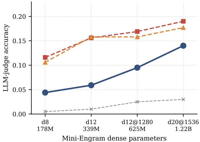
(b) Qwen2.5-14B LLM-as-judge
