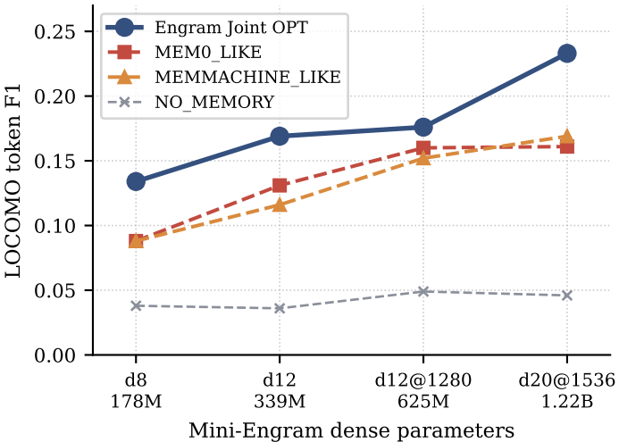
(a) token-F1 metric
