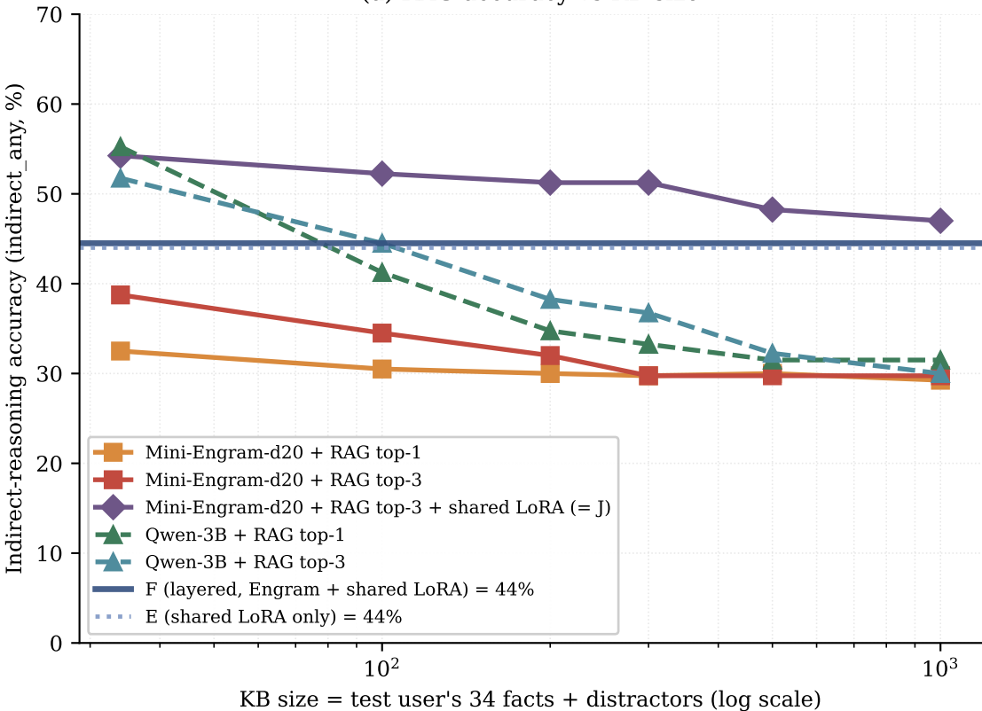
(a) RAG accuracy vs KB size
