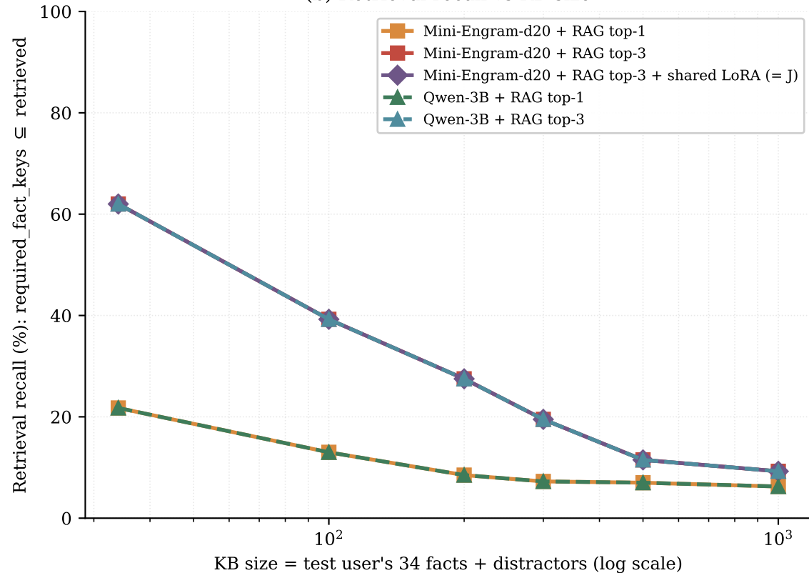
(b) Retrieval recall vs KB size
