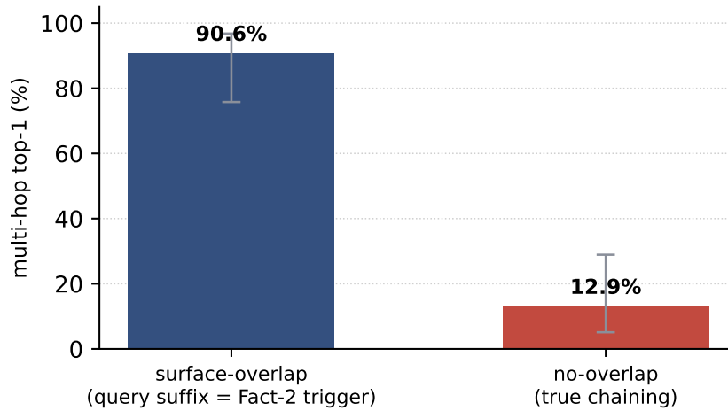
Figure 15. Multi-hop reasoning over Engram-inserted facts ( n=63 chained pairs on Mini-Engram-d20, two OPT-15 insertions per item). Per-fact direct recall is 99.2% (both facts are insertable), so the gap is chaining, not insertion. When the query’s suffix N-gram coincides with Fact-2’s trigger, the gate fires and recall is 90.6%; when true chaining is required, it collapses to 12.9% (Wilson 95% CIs shown). The gate is a surface-N-gram hash—it matches, it does not compose.
