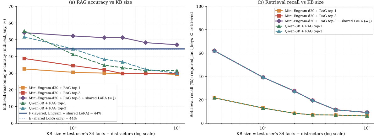
Figure 10. Indirect-reasoning accuracy and retrieval recall vs. KB size ( n=20 users, 20 indirect probes each; KB = test user’s 34 facts + distractors sampled from the 30-user schema-family pool, log x -axis, N \in \{34, 100, 200, 300, 500, 1000\} ). (a) F (layered, horizontal solid line at 44%) is invariant to KB size; the retrieval-based conditions degrade monotonically. Naive RAG and Qwen-3B + RAG fall below F at KB \geq 100 ; at KB=1000 the gap is 14 pp. J (RAG top-3 + shared LoRA) is the most robust to KB growth (54% \rightarrow 47%) because the shared reasoning skill compensates when retrieval misses, though its lead over F shrinks from 10 pp to 3 pp across the sweep. (b) Retrieval recall (fraction of probes where the retrieved set covers all gold required_fact_keys) drops by 7\times for top-3 (62% \rightarrow 9%) between KB=34 and KB=1000, which is the mechanistic driver of (a).
