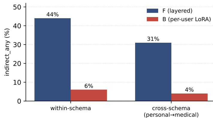
Figure 36. The layered claim survives a personal → medical schema shift (shared LoRA trained on personal-schema users, tested on medical-schema users). F’s indirect_any decays from 44% to 31% (a realistic 30% relative drop) while per-user LoRA B goes 6% → 4%, so F’s lead over B is preserved ( 7.4\times \rightarrow 7.6\times ); locality is unchanged ( \Delta bpb(F)=\Delta bpb(E)=+0.386 ). The Stage-A recite-then-reason recipe, by contrast, collapsed 90% cross-schema (Section 3).
