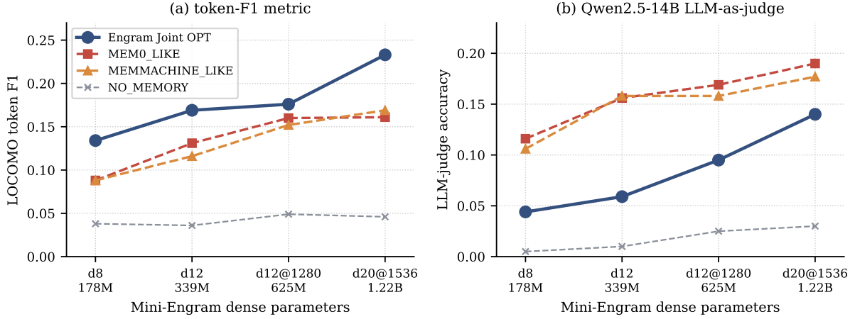
Figure 12. Locomo single-hop, full 10 conversations, scaling with Mini-Engram dense size. (a) Token-F1: User-as-Engram Joint OPT (blue) beats every retrieval baseline at every scale. (b) LLM-judge accuracy (Qwen2.5-14B-Instruct): the ranking flips—retrieval baselines (MEM0_LIKE, MEMMACHINE) beat Joint OPT by 0.05–0.10 because token-F1 over-credits Engram for the correct first answer token despite a noisy continuation.
