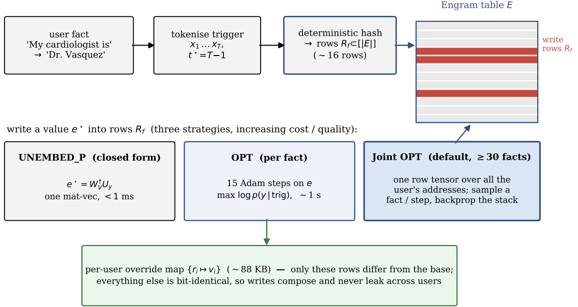
Figure 6. Inserting a user fact into the Engram. A fact is reduced to where and what : the trigger’s suffix N -gram hashes to a sparse set of row addresses R_f ( where ), and one of three strategies writes a value e^* into those rows ( what ). UNEMBED_P solves for e^* in closed form; OPT takes a few gradient steps per fact; Joint OPT—our default beyond \sim 30 facts/user—optimises all of the user’s rows together so they do not interfere. The result is a per-user override map of \sim 88 KB; every row outside R_f , and the entire backbone, is left bit-identical.
