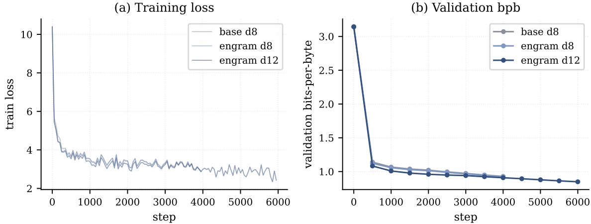
Figure 25. Mini-Engram pretraining curves. Engram d8 reaches lower validation bpb than base d8 at iso-FLOPs (matching the paper’s finding at much smaller scale); engram d12 is substantially better thanks to the larger backbone and longer training.
