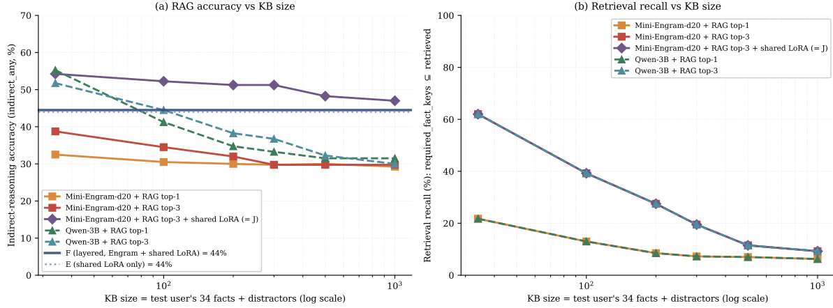
Figure 18. Indirect-reasoning accuracy and retrieval recall vs. KB size ( n=20 users, 20 indirect probes each; KB = test user’s 34 facts + distractors sampled from the 30-user schema-family pool, log x -axis, N \in \{34, 100, 200, 300, 500, 1000\} ). (a) F (layered, horizontal solid line at 44%) is invariant to KB size; the retrieval-based conditions degrade monotonically. Naive RAG and Qwen-3B + RAG fall below F at KB \geq 100 ; at KB=1000 the gap is 14 pp. J (RAG top-3 + shared LoRA) is the most robust to KB growth (54% \rightarrow 47%) because the shared reasoning skill compensates when retrieval misses, though its lead over F shrinks from 10 pp to 3 pp across the sweep. (b) Retrieval recall (fraction of probes where the retrieved set covers all gold required_fact_keys) drops by 7\times for top-3 (62% \rightarrow 9%) between KB=34 and KB=1000, which is the mechanistic driver of (a).
