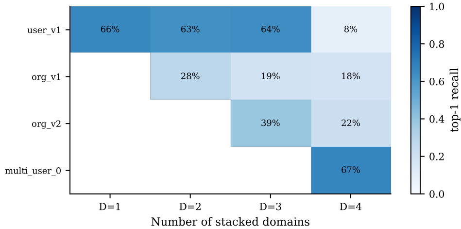
Figure 28. Multi-domain additive composition heatmap. Each cell shows per-domain top-1 recall when D domains are stacked. Heavy degradation when domains share trigger templates (high address overlap). Disjoint-template domains (corp + user, demonstrated in main text) compose without loss.
