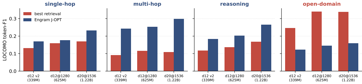
Figure 13. Locomo category breakdown (token-F1), Engram Joint OPT (blue) vs. the best retrieval baseline (red; max of MEM0_LIKE and MEMMACHINE_LIKE) across three dense scales. Engram wins single-hop, multi-hop, and reasoning at every scale—the per-fact (question, answer) loss encodes the question→answer map that retrieval must chain across evidence sentences—but loses open-domain, where the answer is a verbatim span of an unseen evidence sentence that a single-token bias cannot reconstruct. Full numbers in Appendix Table 3.
