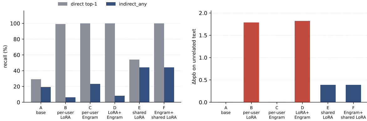
Figure 16. The six parametric conditions on n=20 test users (Mini-Engram-d20, seed S0). Left: F (Engram + shared LoRA) matches per-user LoRA’s direct recall (100% vs. 99%) while delivering 7.4\times its indirect_any (44% vs. 6%); neither the per-user Engram (C, no skill) nor the shared LoRA alone (E, never saw the user’s facts) suffices. Right: F adds zero contamination on top of the shared skill ( \Delta\text{bpb} + 0.386 = \text{E} ), while per-user LoRA (B) and the naive LoRA+Engram stack (D) pay +1.78/+1.82 . RAG conditions (G–J) appear in Figure 17; 3 seeds in Appendix P (3-seed mean F 41%, B 7%).
