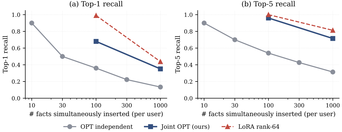
Figure 9. Within-user fact-density: top-1 (left) and top-5 (right) recall vs. number of facts inserted simultaneously into one user’s override map. Joint OPT (blue) closes most of the gap to LoRA rank-64 (red dashed) at 161\times less storage (88 KB vs. 14.2 MB at 100 facts).
