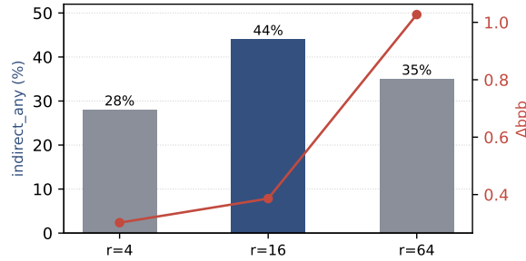
Figure 34. Shared-LoRA rank ablation (layered F, n=20 ). F preserves 100% direct recall at every rank; indirect_any peaks at r=16 (44%) while contamination grows with rank. The r=64 surprise: 4\times the capacity gives worse reasoning (35%) at 2.7\times the contamination, plausibly because capacity exceeds what the 510-sample shared corpus can constrain.
