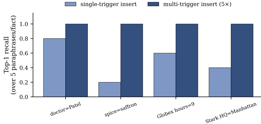
Figure 27. Paraphrase generalisation across 4 facts \times 5 paraphrases each. Single-trigger insertion gets 50% top-1 for free (suffix N-gram overlap); multi-trigger insertion (insert at all 5 paraphrases) gets 100% at 5 \times the per-fact OPT cost.
