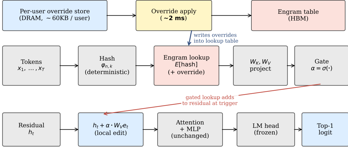
Figure 8. EngramServer architecture. Per user, an override map of (row_idx, row_vector) pairs lives in DRAM. On each request, the server saves the originals at the affected addresses ( \sim 2 ms), writes the user’s overrides, runs the forward pass, then restores. The Engram lookup at the configured layer transparently sees the override values; the gate fires only at the trigger N-gram. There is no router and no graph rewrite.
