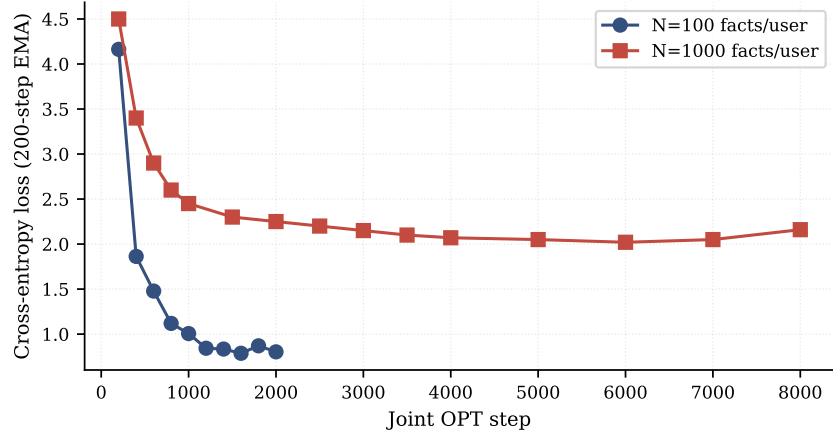
Figure 30. Joint OPT convergence on Mini-Engram-d12. At 100 facts/user, loss converges to 0.8 within 1500 steps; at 1000 facts, loss saturates around 2.0 due to higher within-user fact-density interference (Section 6.2).
