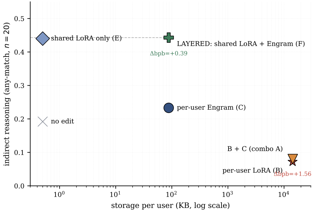
Figure 35. Cost-quality trade-off for the layered architecture (Section 7). Same Mini-Engram-d20 base, n=20 test users, six method combinations. F (LAYERED) gives the best trade-off: it matches the highest indirect-reasoning accuracy (44% indirect_any) at low storage (88 KB/user) and low contamination ( \Delta bpb +0.39 ). F beats per-user LoRA (B) on every measure. The naive combination (B+C, the “add Engram on top of LoRA” baseline) is beaten too.
