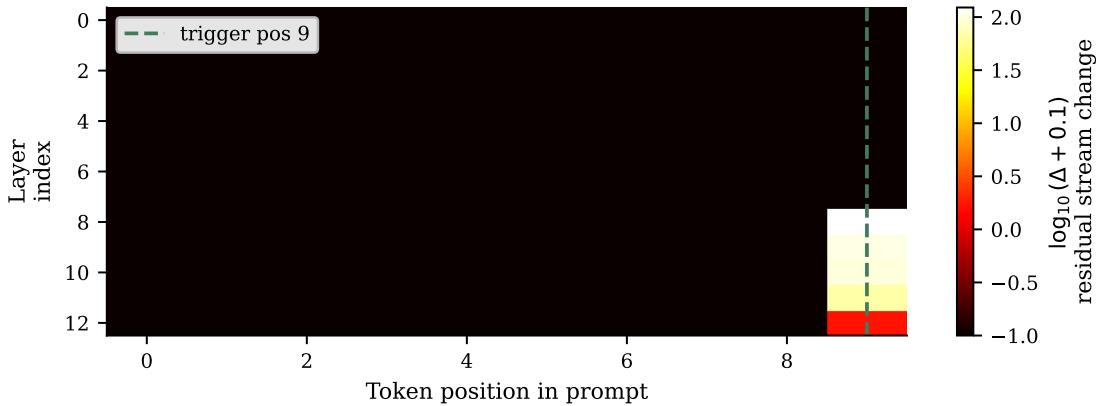
Figure 7. Engram surgical insertion is spatially perfect. Heatmap of \|x_{\text{after}}^{(\ell)} - x_{\text{before}}^{(\ell)}\| for a UNEMBED_P insertion at the last Engram layer ( L_{\text{eng}}=7 , Mini-Engram-d12). The diff is exactly 0.000 at every position before L_{\text{eng}} (causality) and at every non-trigger position after L_{\text{eng}} , through 5 subsequent attention/MLP layers. Compare with LoRA, where every position in every forward sees the global delta.
