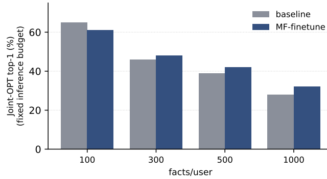
Figure 21. Multi-fact-in-the-loss finetune vs. baseline d12@1280 on the Joint-OPT density curve (matched OPT-step schedule). At a fixed inference budget MF improves recall at high density (+14% relative at n=1000 , 8k steps). With the budget unpinned (12k steps) both reach \sim 34.5\% at n=1000 : MF accelerates convergence rather than raising the asymptotic ceiling. val_bpb is preserved (0.774 vs. 0.770).
