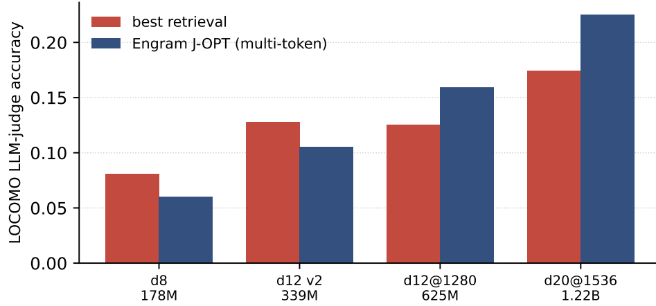
Figure 23. LOCOMO single-hop under an LLM judge (Qwen2.5-14B), matched multi-token pipeline. First-token OPT lets token-F1 over-credit Engram for a correct first token over a noisy continuation (Figure 22); training the full answer with multi-token Joint-OPT fixes this and overtakes the best retrieval baseline from d12@1280 upward (+27% at 625 M, +29% at 1.22 B). Below that cross-over the dense backbone is too small for the continuation to fall into place after the Engram-anchored prefix.
