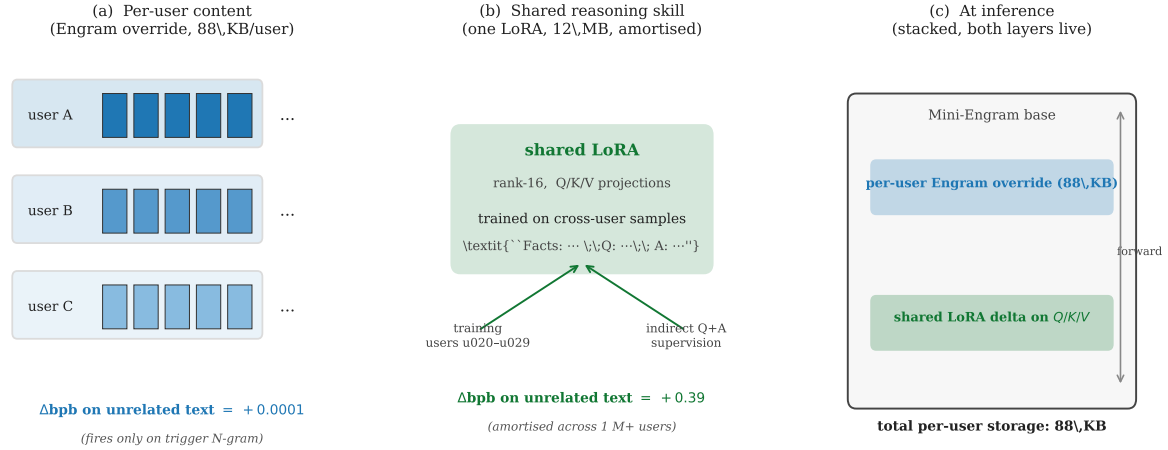
Figure 15. The layered architecture splits personal memory by who owns it and how often it changes. (a) Per-user content is a small Engram-row override (88 KB/user) that fires only on its trigger N-gram, so it perturbs unrelated text by \Delta\text{bpb} = +0.0001 . (b) The shared reasoning skill is a single rank-16 LoRA trained on cross-user indirect-QA samples; its \Delta\text{bpb} = +0.39 contamination is paid once and amortised across all users. (c) At inference both layers are live on the frozen Mini-Engram base: the Engram supplies content via N-gram lookup and the shared LoRA supplies the in-context-reasoning skill, at a total per-user storage cost of 88 KB.
