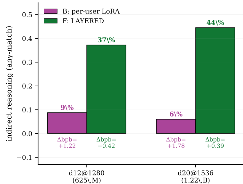
(a) Layered F dominates LoRA B across two Engram sizes
