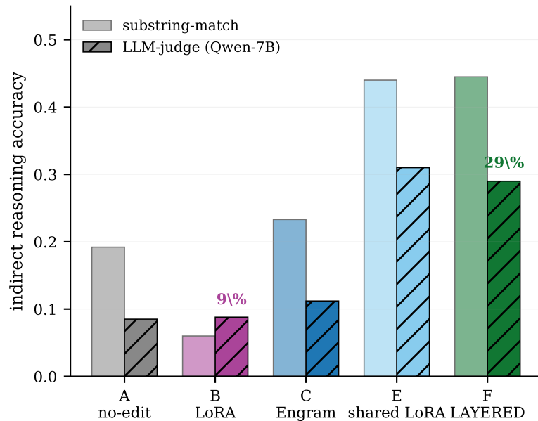
(b) F still beats B under semantic LLM-judge
