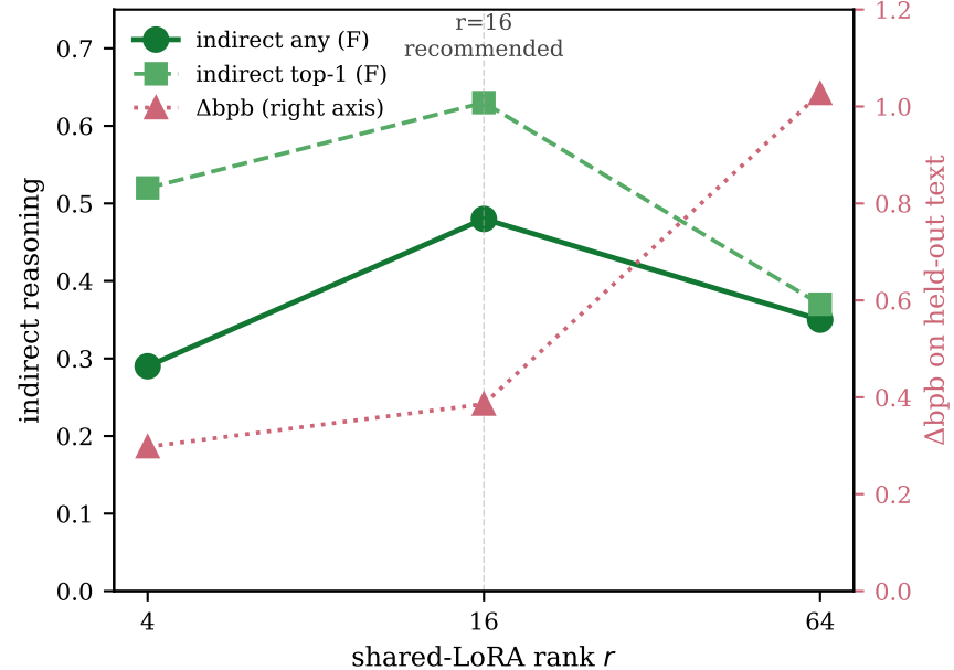
(c) Rank ablation: r=16 is the sweet spot ( r=64 over-parameterises)
