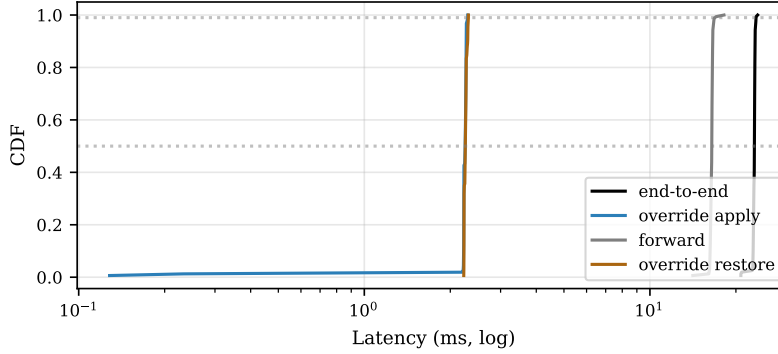
Figure 18: Per-request latency CDF on Mini-Engram-d12 (30 users \times 50 facts \times 600 requests). Override apply (blue) and restore (orange) are both sub-3 ms at p99; the forward pass (grey) dominates total latency (black).
