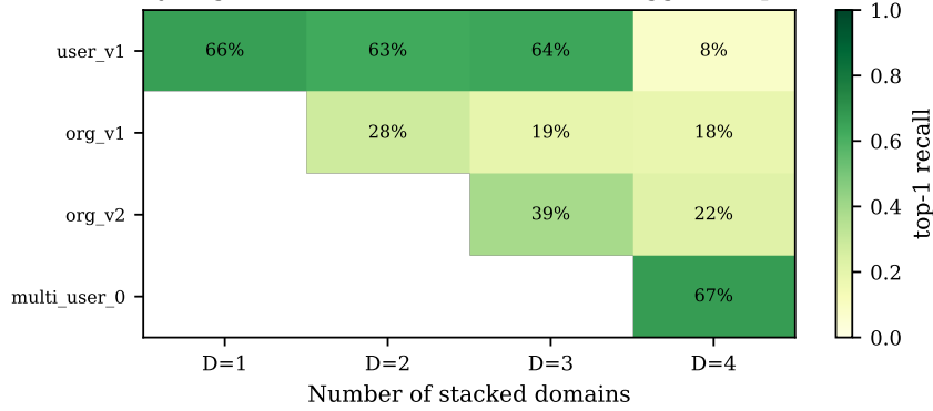
Figure 17: Multi-domain additive composition heatmap. Each cell shows per-domain top-1 recall when D domains are stacked. Heavy degradation when domains share trigger templates (high address overlap). Disjoint-template domains (corp + user, demonstrated in main text) compose without loss.
