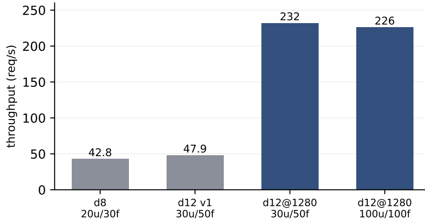
Figure 14. EngramServer throughput across four deployment scales on one idle Blackwell GPU. On the ablation-optimal d12@1280 the server reaches 232 req/s (30 u/50 f) and holds 226 req/s at 100 u/100 f—within 3% as tenants triple—at 4.4 ms p50 latency, a 0.03 ms override apply, 88 KB/user, and 62%/96% top-1/top-5 own-fact recall. Per-request work is independent of tenant count, and cross-user information flow is zero under the apply/restore protocol.
