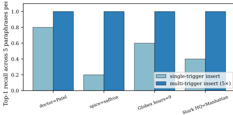
Figure 24. Paraphrase generalisation across 4 facts \times 5 paraphrases each. Single-trigger insertion gets 50% top-1 for free (suffix N -gram overlap); multi-trigger insertion (insert at all 5 paraphrases) gets 100% at 5\times the per-fact OPT cost.
