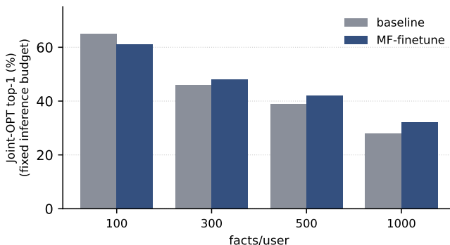
Figure 18. Multi-fact-in-the-loss finetune vs. baseline d12@1280 on the Joint-OPT density curve (matched OPT-step schedule). At a fixed inference budget MF improves recall at high density (+14% relative at n=1000 , 8k steps). With the budget unpinned (12k steps) both reach \sim 34.5\% at n=1000 : MF accelerates convergence rather than raising the asymptotic ceiling. val_bpb is preserved (0.774 vs. 0.770).
