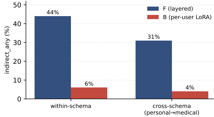
Figure 33. The layered claim survives a personal \rightarrow medical schema shift (shared LoRA trained on personal-schema users, tested on medical-schema users). F’s indirect_any decays from 44% to 31% (a realistic 30% relative drop) while per-user LoRA B goes 6% \rightarrow 4%, so F’s lead over B is preserved ( 7.4\times \rightarrow 7.6\times ); locality is unchanged ( \Delta\text{bpb}(F)=\Delta\text{bpb}(E)=+0.386 ). The Stage-A recite-then-reason recipe, by contrast, collapsed 90% cross-schema (Section 3).
