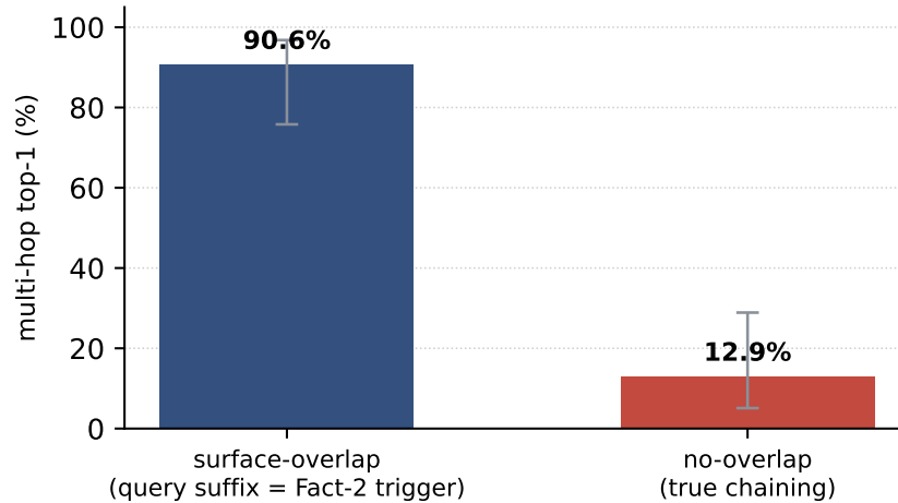
Figure 12. Multi-hop reasoning over Engram-inserted facts ( n=63 chained pairs on Mini-Engram-d20, two OPT-15 insertions per item). Per-fact direct recall is 99.2% (both facts are insertable), so the gap is chaining, not insertion. When the query’s suffix N-gram coincides with Fact-2’s trigger, the gate fires and recall is 90.6%; when true chaining is required, it collapses to 12.9% (Wilson 95% CIs shown). The gate is a surface-N-gram hash—it matches, it does not compose.
