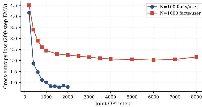
Figure 26. Joint OPT convergence on Mini-Engram-d12. At 100 facts/user, loss converges to 0.8 within 1500 steps; at 1000 facts, loss saturates around 2.0 due to higher within-user fact-density interference (Section 5.2).
