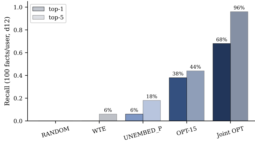
Figure 20. Top-1 and top-5 recall at 100 facts/user, Mini-Engram-d12. RANDOM (control) confirms our signal isn’t noise; UNEMBED_P alone is too weak; OPT-15 helps; Joint OPT closes most of the gap to full LoRA fine-tuning at 161\times less storage.
