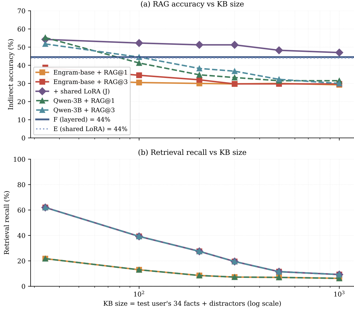
Figure 14. Indirect-reasoning accuracy and retrieval recall vs. KB size ( n=20 users, 20 indirect probes each; KB = test user’s 34 facts + distractors sampled from the 30-user schema-family pool, log x -axis, N \in \{34, 100, 200, 300, 500, 1000\} ). (a) F (layered, horizontal solid line at 44%) is invariant to KB size; the retrieval-based conditions degrade monotonically. Naive RAG and Qwen-3B + RAG fall below F at KB \geq 100 ; at KB=1000 the gap is 14 pp. J (RAG top-3 + shared LoRA) is the most robust to KB growth (54% \rightarrow 47%) because the shared reasoning skill compensates when retrieval misses, though its lead over F shrinks from 10 pp to 3 pp across the sweep. (b) Retrieval recall (fraction of probes where the retrieved set covers every fact the question needs) drops by 7\times for top-3 (62% \rightarrow 9%) between KB=34 and KB=1000, which is the mechanistic driver of (a).
