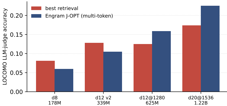
Figure 17. Locomo single-hop under an LLM judge (Qwen2.5-14B), matched multi-token pipeline. First-token OPT lets token-F1 over-credit Engram for a correct first token over a noisy continuation (Figure 16); training the full answer with multi-token Joint-OPT fixes this and overtakes the best retrieval baseline from d12@1280 upward (+27% at 625 M, +29% at 1.22 B). Below that cross-over the dense backbone is too small for the continuation to fall into place after the Engram-anchored prefix.
