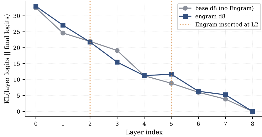
Figure 18. LogitLens KL by layer (Mini-Engram-d8 vs. base-d8). Engram converges faster at layer 3 (–3.66 KL gap), confirming Cheng et al.’s effective-deepening claim at our scale (stage 4 of the mechanism above).
