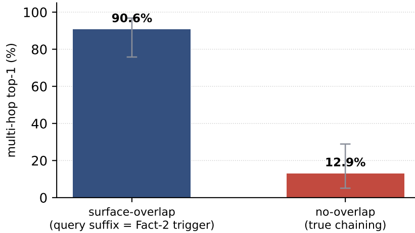
Figure 11. Multi-hop reasoning over Engram-inserted facts ( n=63 chained pairs on Mini-Engram-d20, two OPT-15 insertions per item). Per-fact direct recall is 99.2% (both facts are insertable), so the gap is chaining, not insertion. When the query’s suffix N-gram coincides with Fact-2’s trigger, the gate fires and recall is 90.6%; when true chaining is required, it collapses to 12.9% (Wilson 95% CIs shown). The gate is a surface-N-gram hash—it matches, it does not compose.
