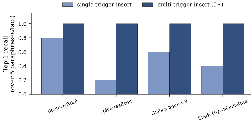
Figure 21. Paraphrase generalisation across 4 facts \times 5 paraphrases each. Single-trigger insertion gets 50% top-1 for free (suffix N-gram overlap); multi-trigger insertion (insert at all 5 paraphrases) gets 100% at 5\times the per-fact OPT cost.
