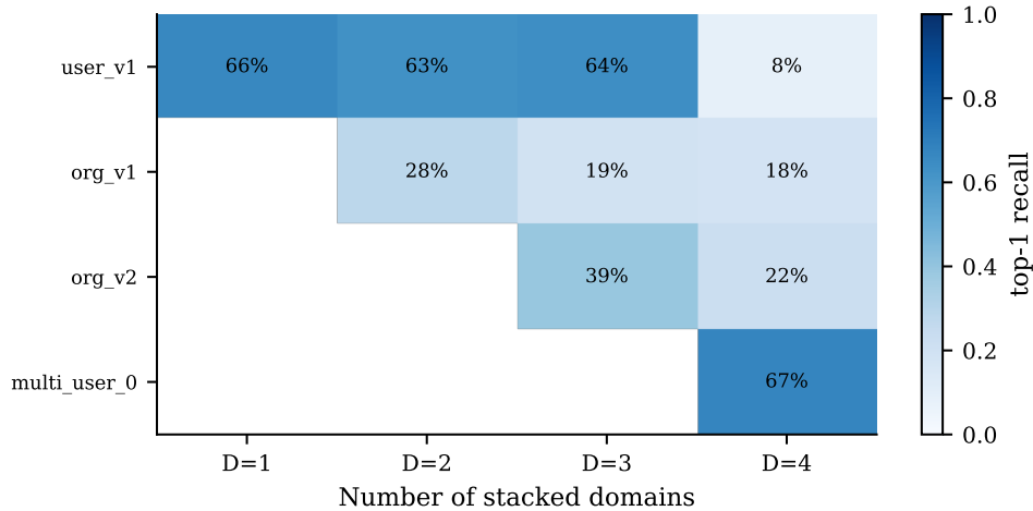
Figure 22. Multi-domain additive composition heatmap. Each cell shows per-domain top-1 recall when D domains are stacked. Heavy degradation when domains share trigger templates (high address overlap). Disjoint-template domains (corp + user, demonstrated in main text) compose without loss.
