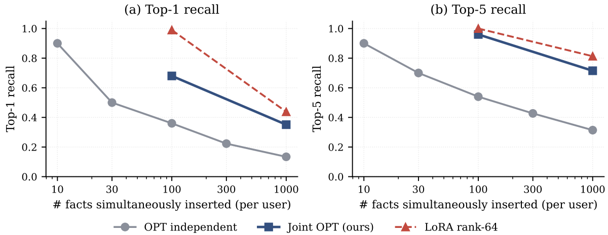
Figure 27. Within-user fact-density: top-1 (left) and top-5 (right) recall vs. number of facts inserted simultaneously into one user’s override map. Joint OPT (blue) closes most of the gap to LoRA rank-64 (red dashed) at 161\times less storage (88 KB vs. 14.2 MB at 100 facts).
