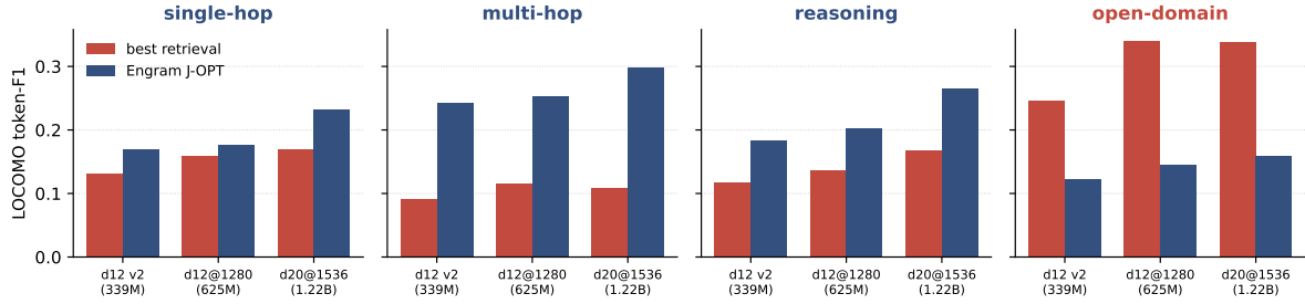
Figure 15. Locomo category breakdown (token-F1), Engram Joint OPT (blue) vs. the best retrieval baseline (red; max of MEM0_LIKE and MEMMACHINE_LIKE) across three dense scales. Engram wins single-hop, multi-hop, and reasoning at every scale—the per-fact (question, answer) loss encodes the question→answer map that retrieval must chain across evidence sentences—but loses open-domain, where the answer is a verbatim span of an unseen evidence sentence that a single-token bias cannot reconstruct.
