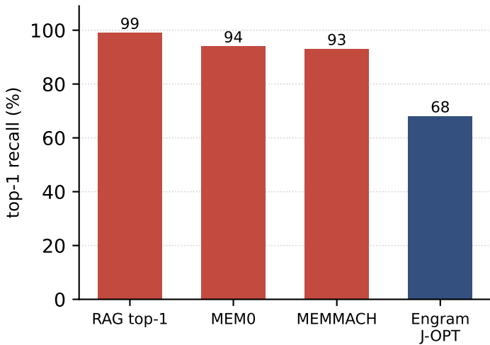
Trigger-exact query
