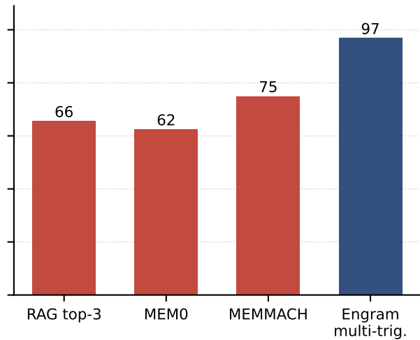
Paraphrased query
