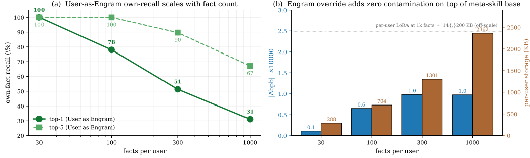
Figure 6: Density scaling on Mini-Engram-d20 with the meta-skill foundational model. (a) Own-fact recall: top-1 decays as expected with more facts/user (100% → 78% → 51% → 31%), but top-5 stays high through 300 facts (90%) and degrades gracefully to 67% at 1,000 facts. (b) The headline architectural finding: adding per-user Engram content on top of the meta-skill base adds zero additional contamination — |\Delta\text{bpb}| is at most 0.0001 across all densities, indistinguishable from noise. Per-user storage scales linearly with rows touched (288 → 704 → 1,301 → 2,362 rows, equivalently 288 KB → 2.4 MB at 1k facts), still \sim 6\times smaller than per-user LoRA’s 14.2 MB at the same fact-count.
