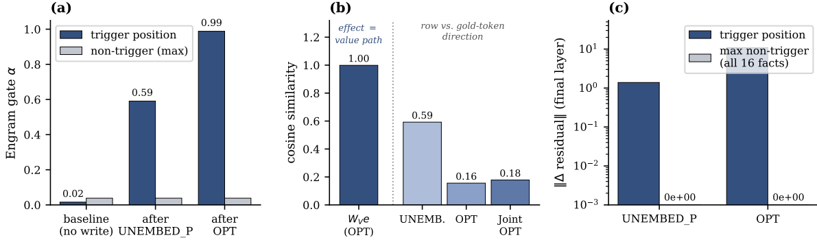
Figure 8. The mechanism on the trained model (Mini-Engram-d20, 16 facts). (a) The write opens its own gate: the trigger-position gate \alpha rises from 0.02 to 0.99 (OPT) while non-trigger positions stay at 0.04. (b) The deployed row’s residual change is cosine 0.999 to its value-path projection W_{Ve} (left bar); what the row encodes relative to the gold token’s unembedding is exact for the closed-form solution (0.59) and drifts as gradient OPT/Joint-OPT trade direct gold-alignment for higher recall (0.16–0.18). (c) Exact locality: the maximum non-trigger residual change over all 16 facts is 0.000 for both strategies, versus an order-1 change at the trigger.
