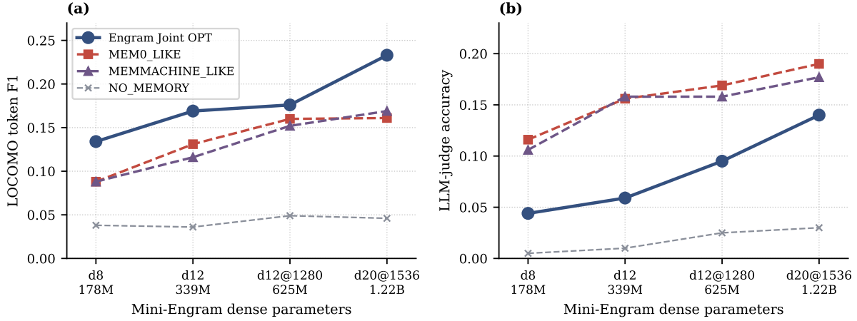
Figure 12. Locomo single-hop, full 10 conversations, scaling with Mini-Engram dense size. (a) Token-F1 : User-as-Engram Joint OPT (blue) beats every retrieval baseline at every scale. (b) LLM-judge accuracy (Qwen2.5-14B-Instruct): the ranking flips—retrieval baselines (MEM0_LIKE, MEMMACHINE) beat Joint OPT by 0.05–0.10 because token-F1 over-credits Engram for the correct first answer token despite a noisy continuation.
