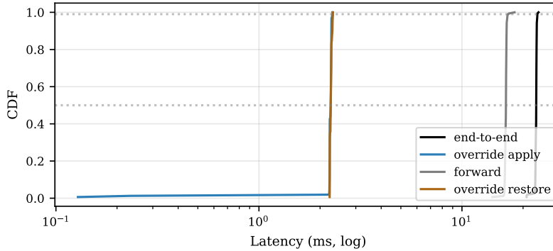
Figure 19: Per-request latency CDF on Mini-Engram-d12 (30 users \times 50 facts \times 600 requests). Override apply (blue) and restore (orange) are both sub-3 ms at p99; the forward pass (grey) dominates total latency (black).
