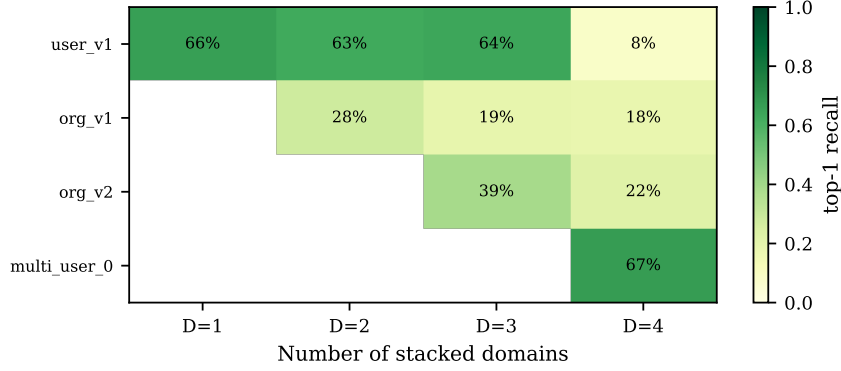
Figure 19: Multi-domain additive composition heatmap. Each cell shows per-domain top-1 recall when D domains are stacked. Heavy degradation when domains share trigger templates (high address overlap). Disjoint-template domains (corp + user, demonstrated in main text) compose without loss.
