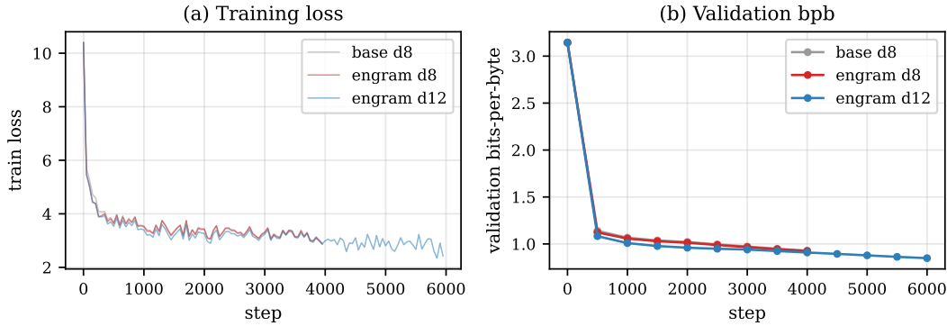
Figure 16: Mini-Engram pretraining curves. Engram d8 reaches lower validation bpb than base d8 at iso-FLOPs (matching the paper’s finding at much smaller scale); engram d12 is substantially better thanks to the larger backbone and longer training.
