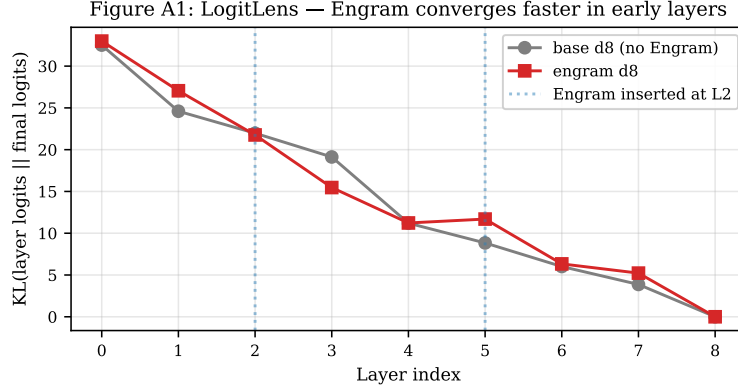
Figure 15: LogitLens KL by layer (Mini-Engram-d8 vs. base-d8). Engram converges faster at layer 3 (−3.66 KL gap), confirming Cheng et al.’s effective-deepening claim at our scale.
