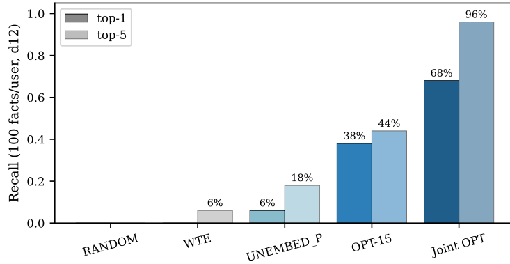
Figure 17: Top-1 and top-5 recall at 100 facts/user, Mini-Engram-d12. RANDOM (control) confirms our signal isn't noise; UNEMBED_P alone is too weak; OPT-15 helps; Joint OPT closes most of the gap to full LoRA fine-tuning at 161\times less storage.
