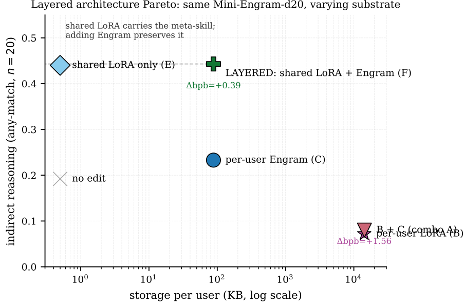
Figure 14: Cost-quality Pareto for the layered architecture (Section 8). Same Mini-Engram-d20 base, n=20 test users, six substrate combinations. F (LAYERED) is on the Pareto frontier : matches the highest indirect-reasoning accuracy (44% indirect-any) at low storage (88 KB/user) and low contamination ( \Delta\text{bpb} +0.39 ). Per-user LoRA (B) is Pareto-dominated by F on every axis. Naive combination (B+C, the “add Engram on top of LoRA” baseline) is also dominated.
