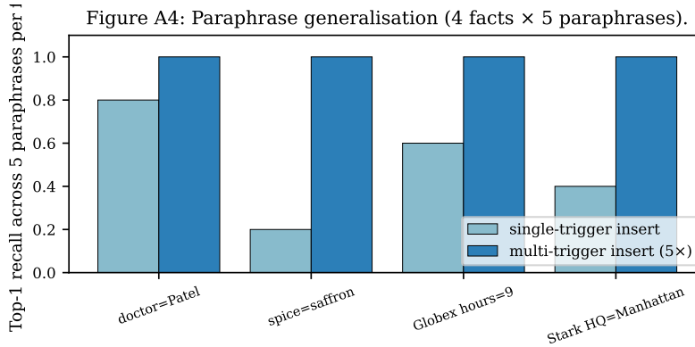
Figure 18: Paraphrase generalisation across 4 facts \times 5 paraphrases each. Single-trigger insertion gets 50% top-1 for free (suffix N-gram overlap); multi-trigger insertion (insert at all 5 paraphrases) gets 100% at 5\times the per-fact OPT cost.
