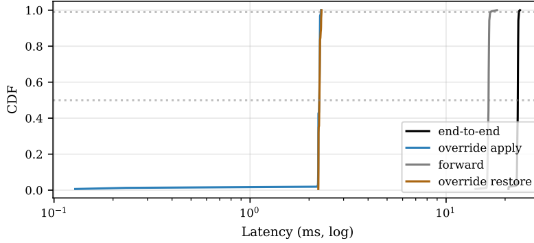
Figure 20: Per-request latency CDF on Mini-Engram-d12 (30 users \times 50 facts \times 600 requests). Override apply (blue) and restore (orange) are both sub-3 ms at p99; the forward pass (grey) dominates total latency (black).
