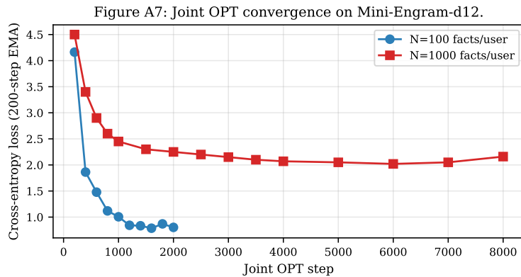
Figure 21: Joint OPT convergence on Mini-Engram-d12. At 100 facts/user, loss converges to 0.8 within 1500 steps; at 1000 facts, loss saturates around 2.0 due to higher within-user fact-density interference (Section 6.2).
