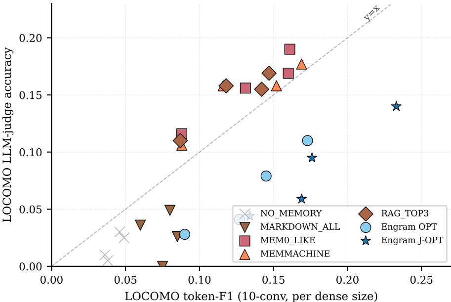
token-F1 vs LLM-judge: Engram OPT systematically over-credited by token-F1
