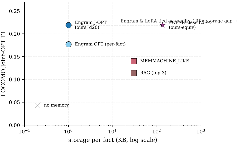
Cost-quality Pareto: same LM (Mini-Engram-d20@1536), varying memory substrate
