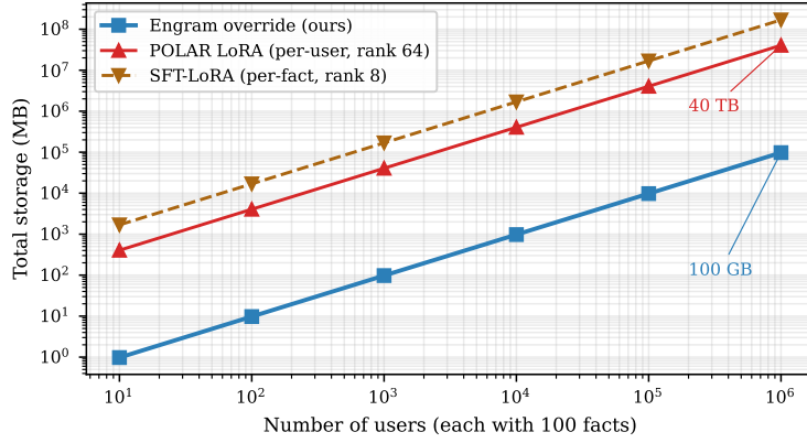
Figure 7: Storage scales linearly with user count for both approaches; Engram override is 200–1700 \times smaller per fact. At 1 M users \times 100 facts/user, Engram storage is 100 GB vs. POLAR LoRA’s 40TB.
