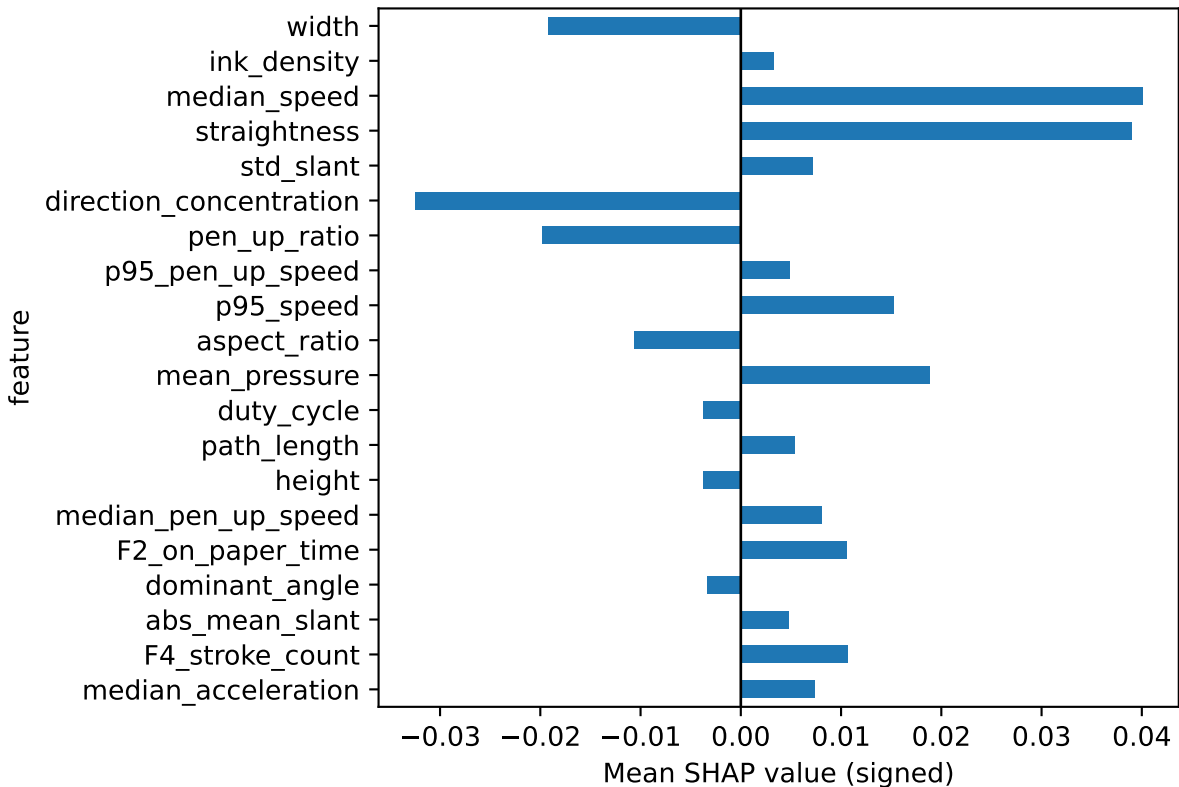
Top 20 Signed SHAP Gradient Boosting - depression
