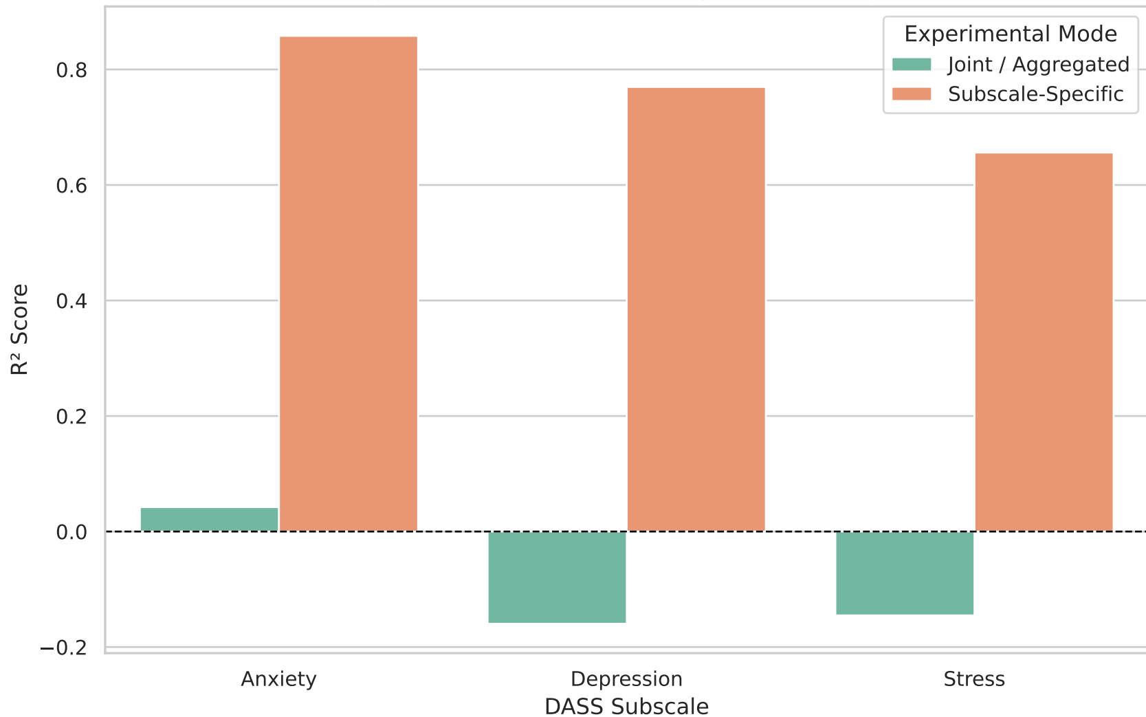
Comparison of Joint vs Subscale-Specific Modeling ( R^2 )
