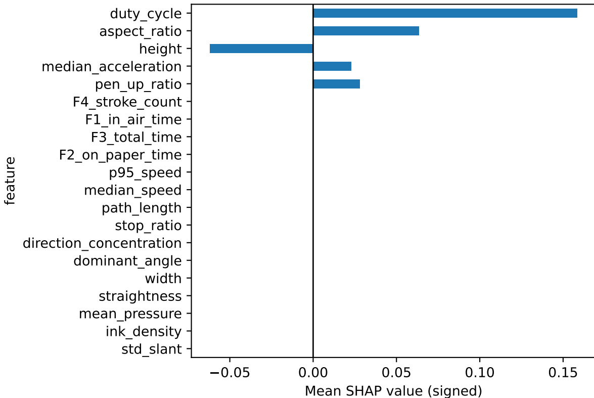
Top 20 Signed SHAP Lasso Regression - anxiety
