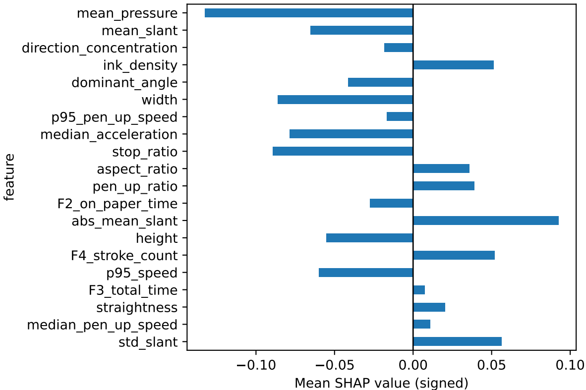
Top 20 Signed SHAP Linear Regression - stress
