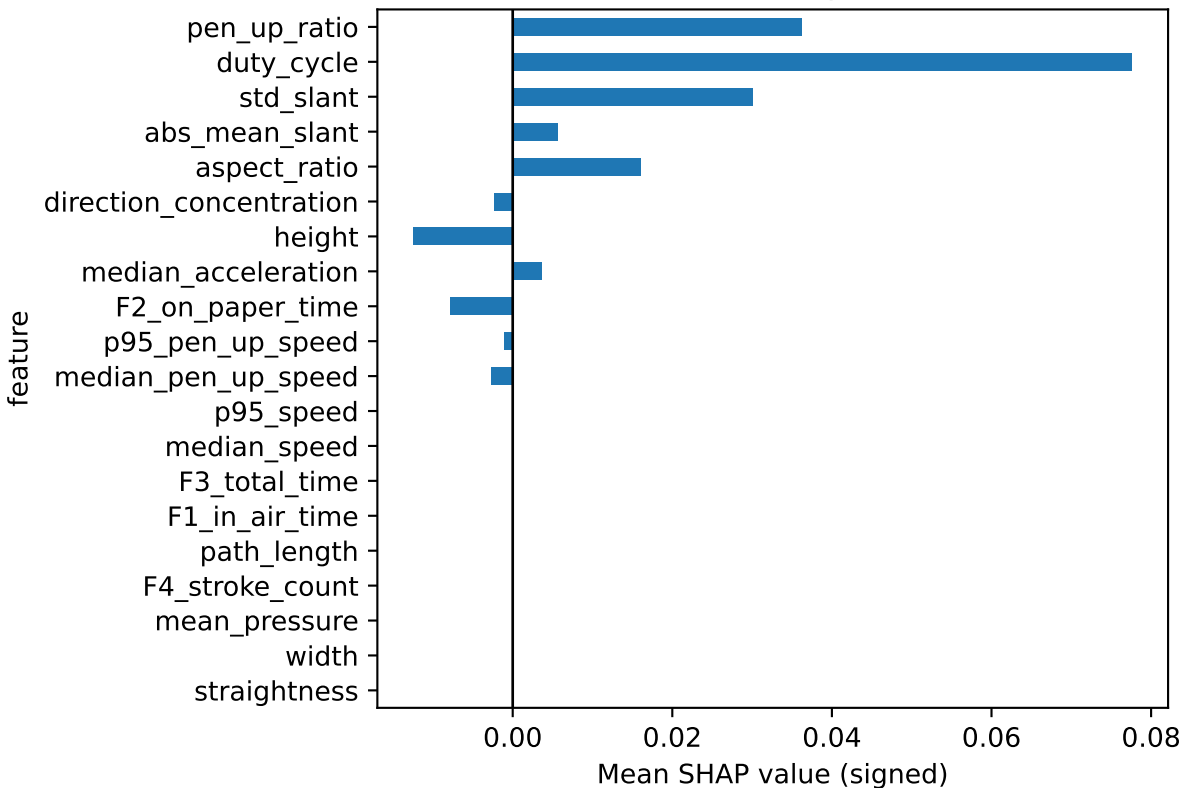
Top 20 Signed SHAP Elastic Net - depression
