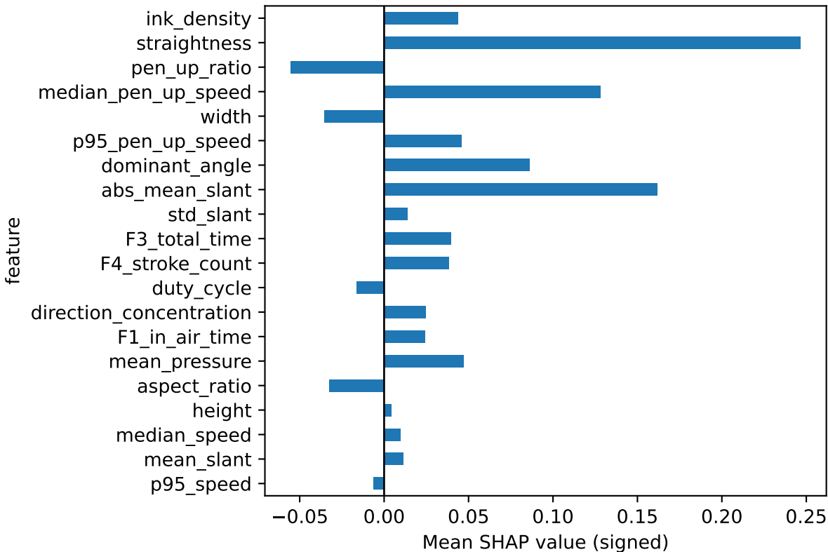
Top 20 Signed SHAP Gradient Boosting - TOTAL_DASS
