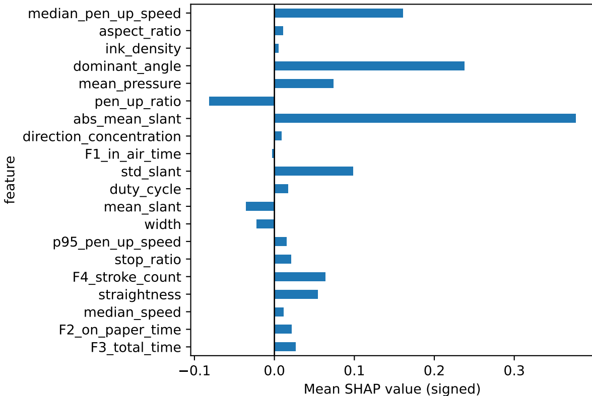
Top 20 Signed SHAP Random Forest - stress
