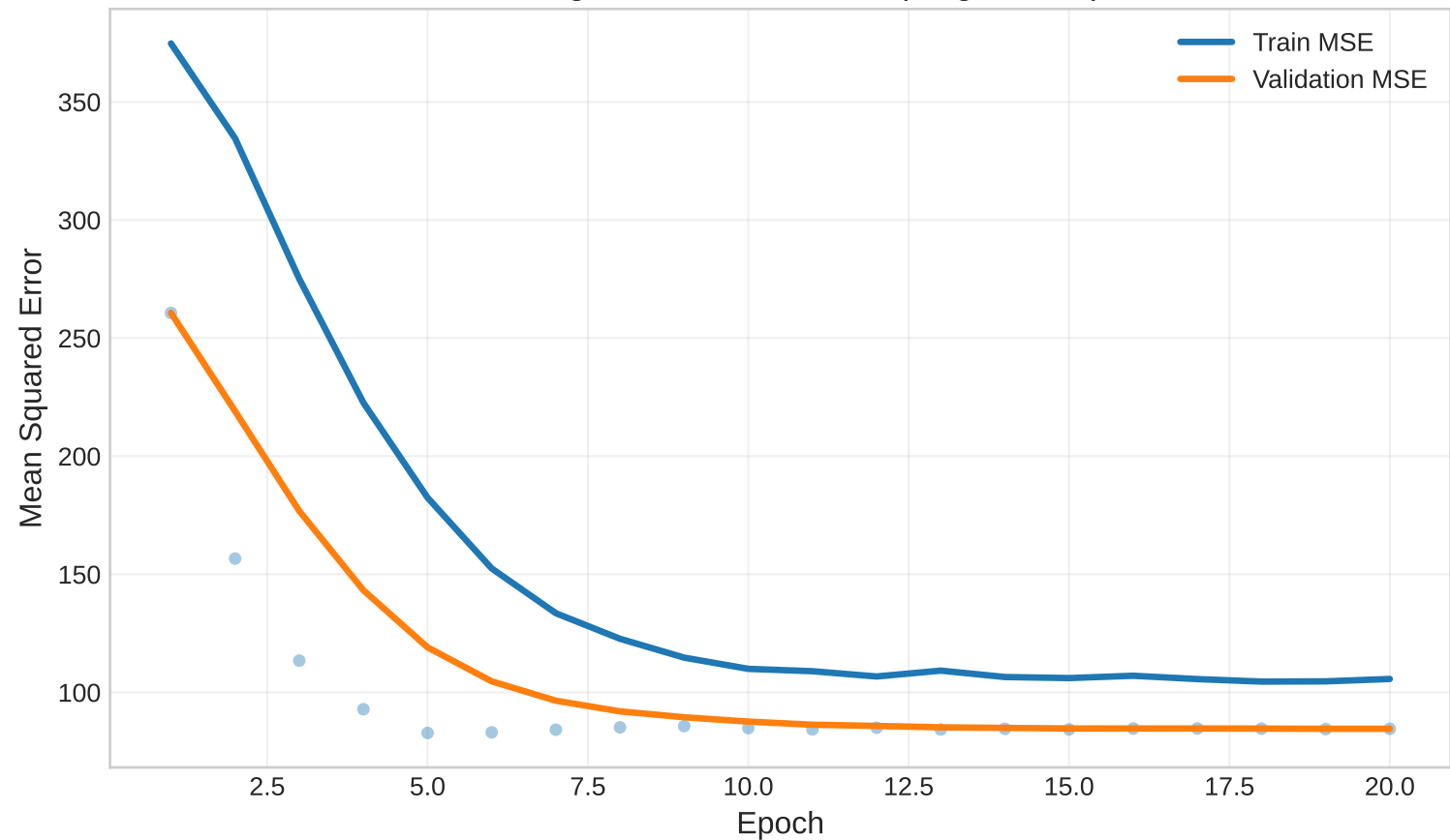
Training vs Validation Loss (Regression)
