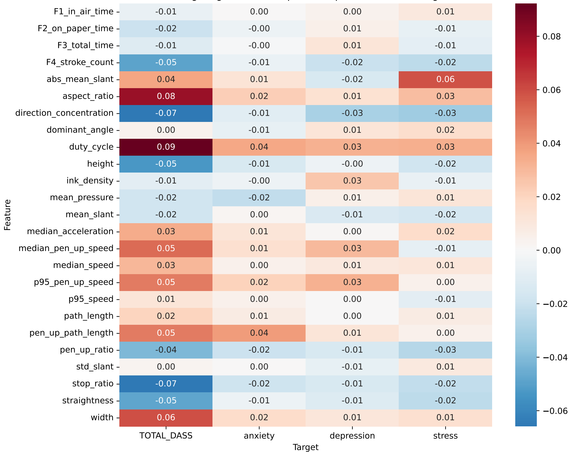
Average Signed SHAP Importance per Feature and Target
