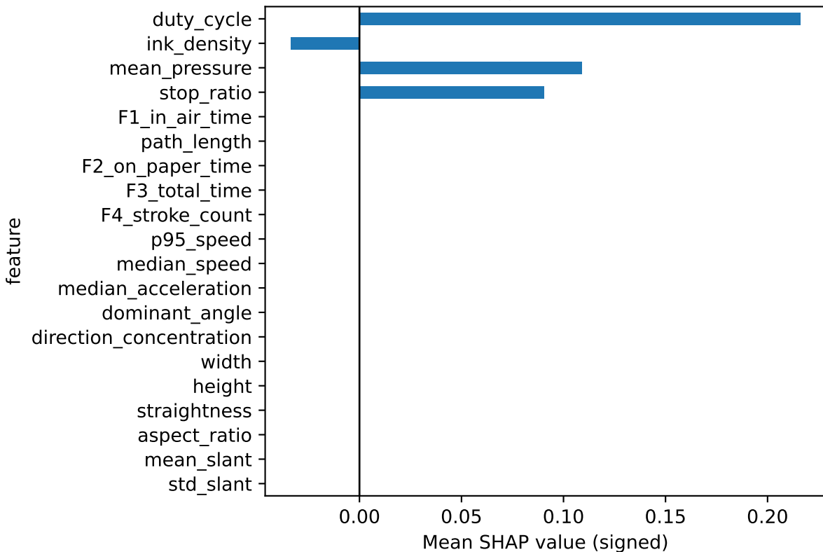
Top 20 Signed SHAP Lasso Regression - stress
