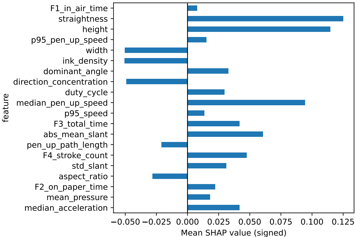
Top 20 Signed SHAP Random Forest - anxiety
