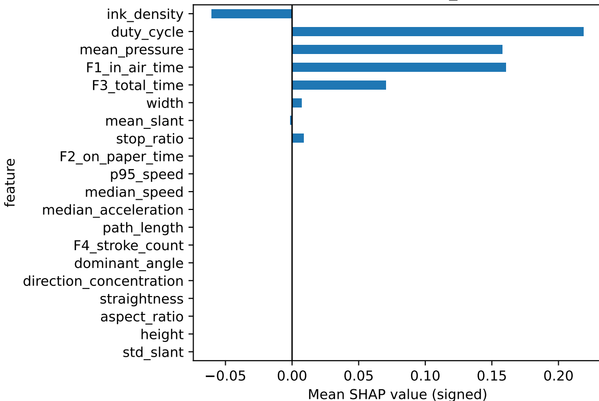
Top 20 Signed SHAP Elastic Net - TOTAL_DASS
