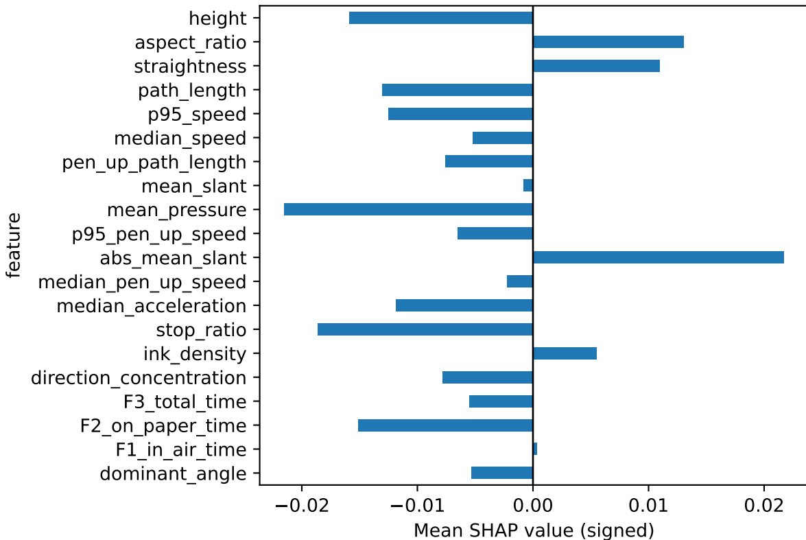
Top 20 Signed SHAP Ridge Regression - stress
