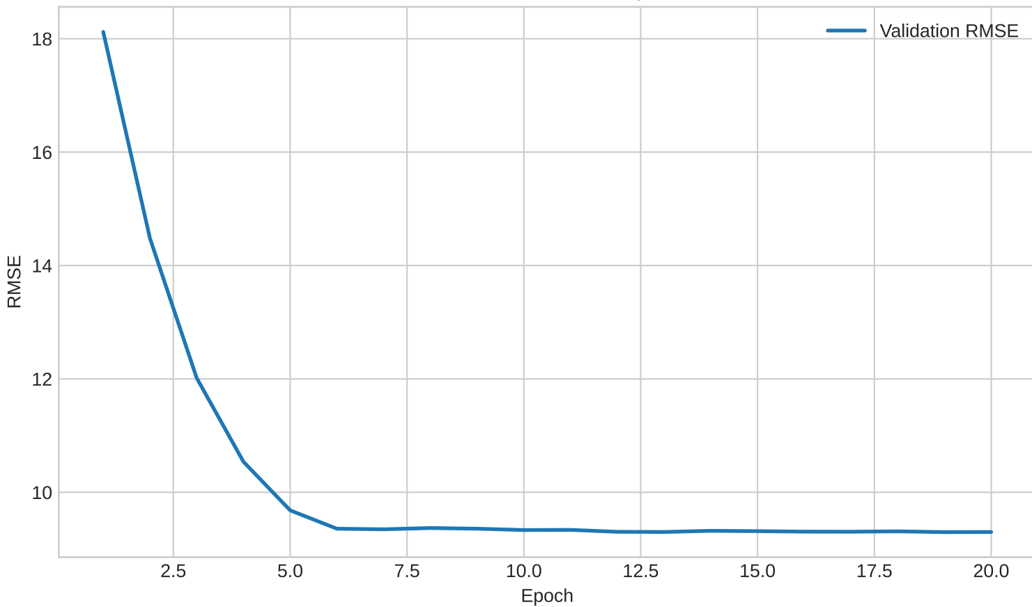
Validation RMSE over Epochs
