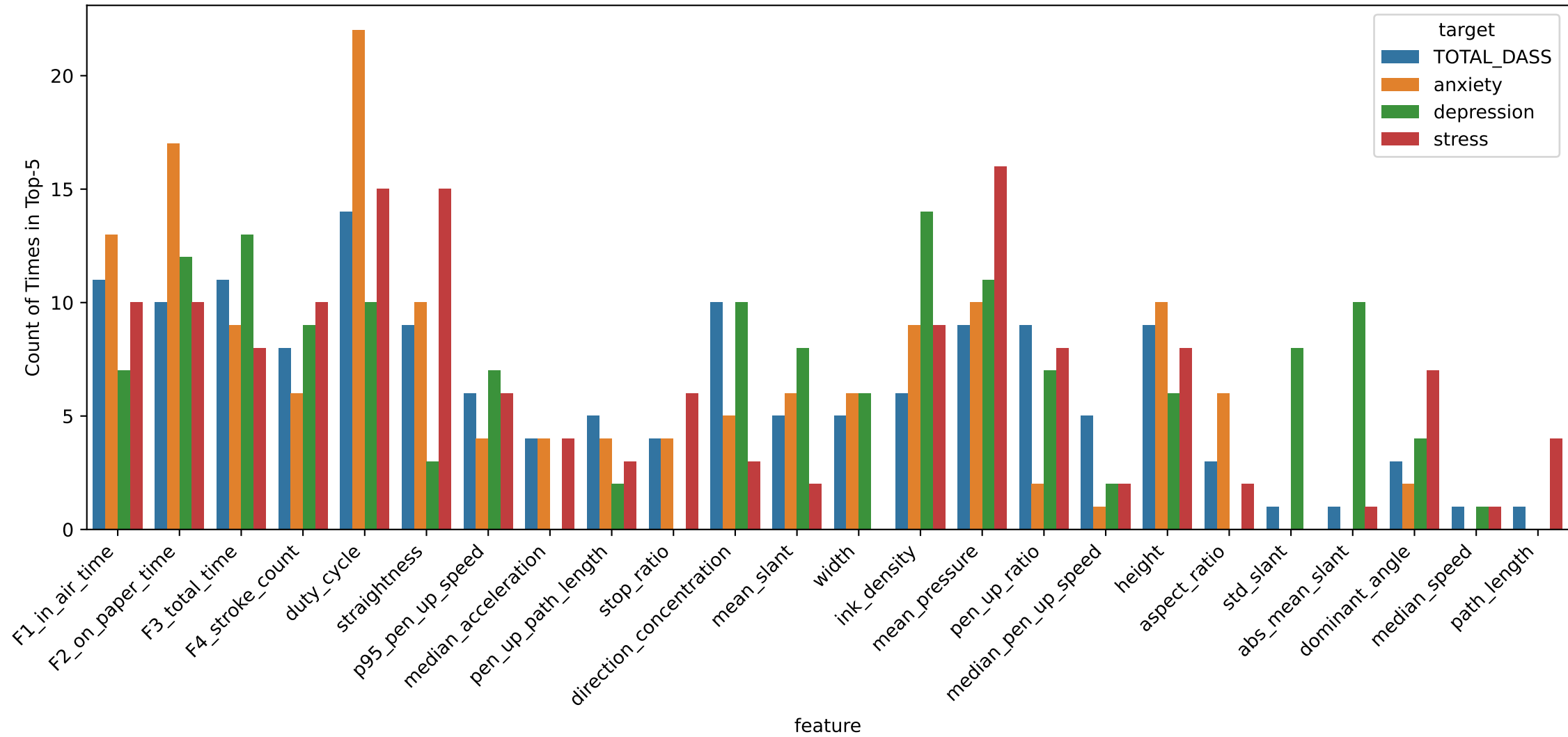
Top-5 SHAP Features Across Models & Tasks
