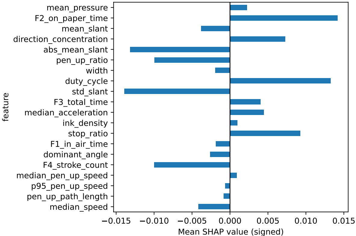
Top 20 Signed SHAP Ridge Regression - anxiety
