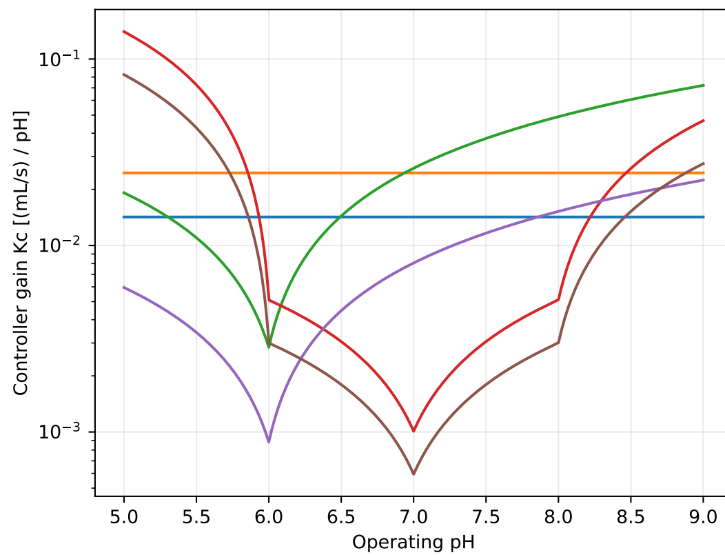
Gain scheduling compensates local process-gain nonlinearity
