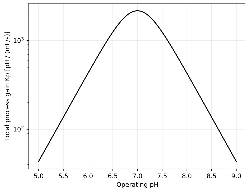
Gain scheduling compensates local process-gain nonlinearity
