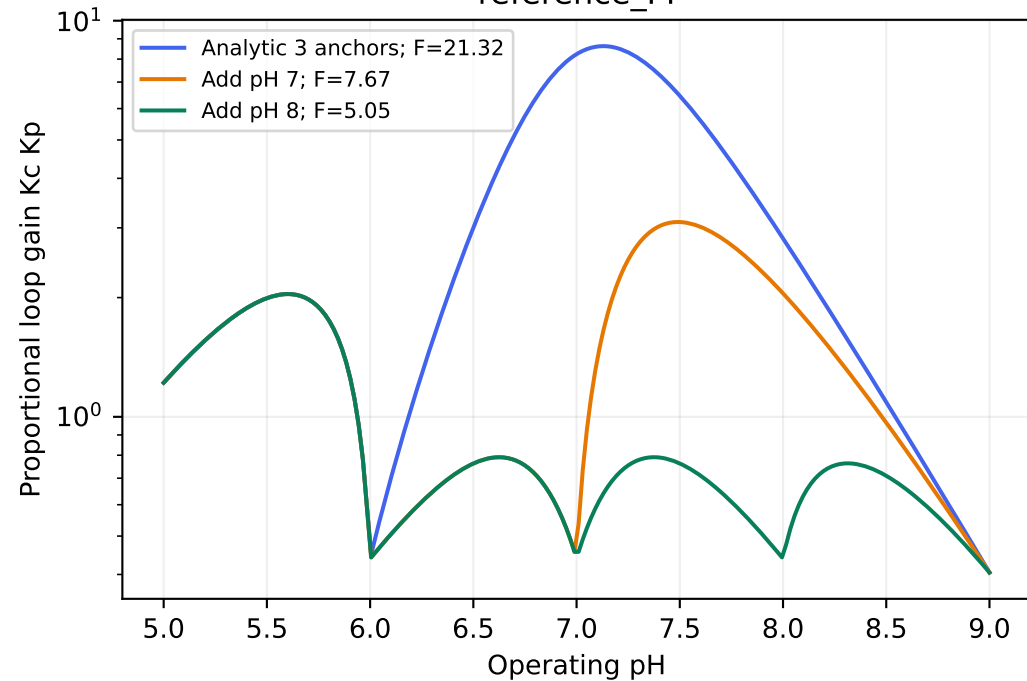
reference_PI
