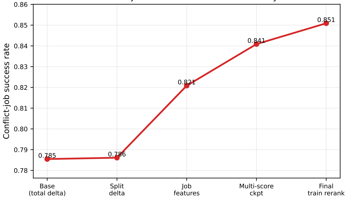
Conflict-job success rate in Ablation Study
