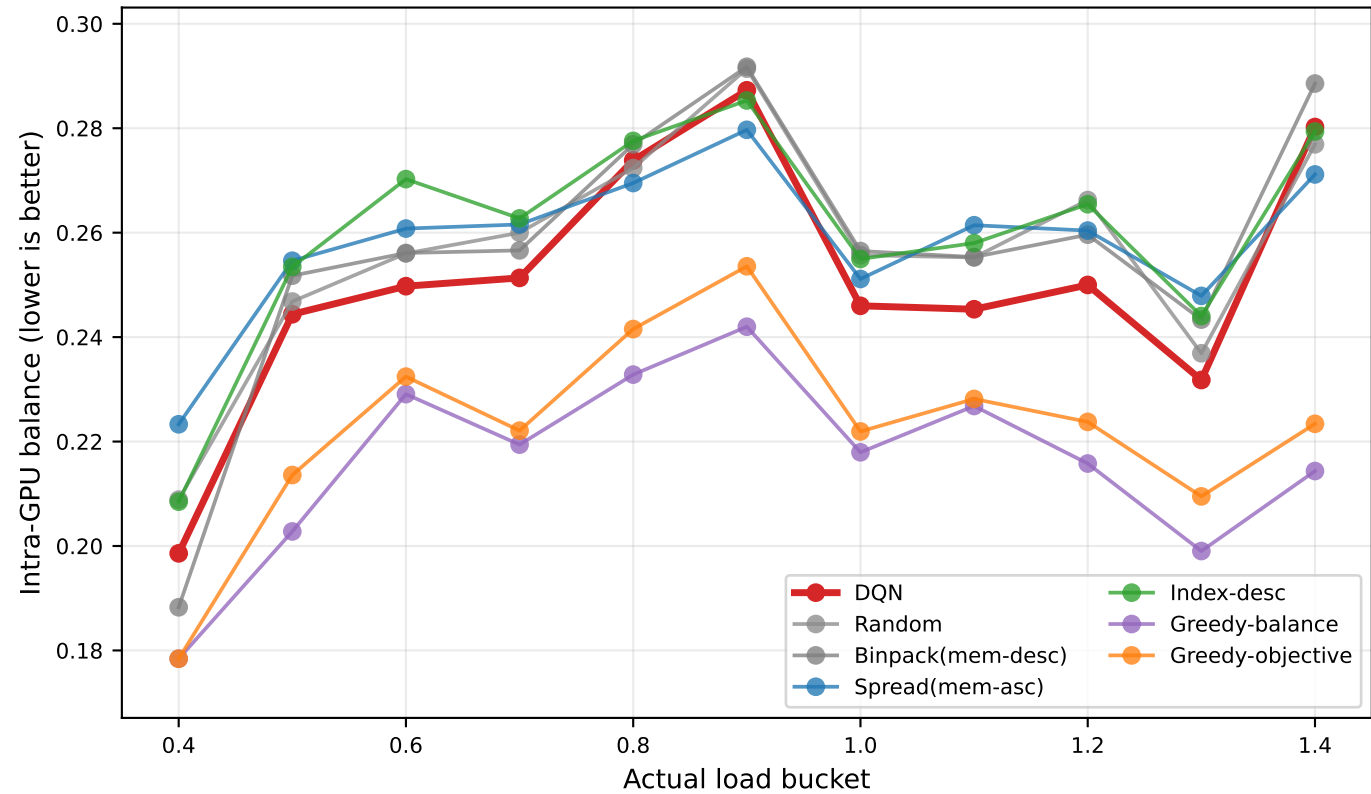
Intra-GPU balance across Load Levels
