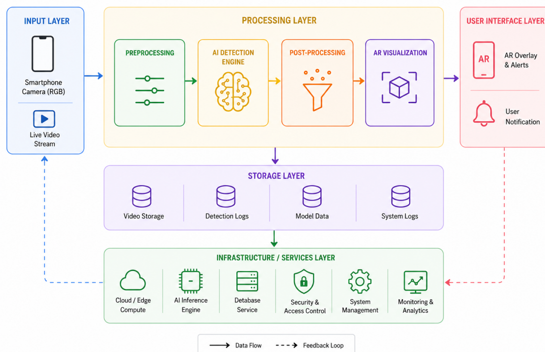
Fig. 4.1: System Architecture
