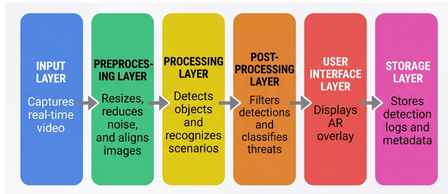
Figure 4.1: System Architecture
