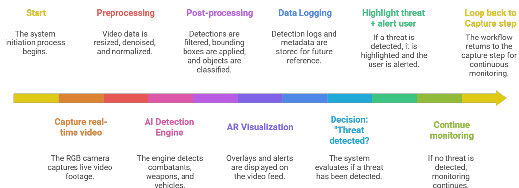
Figure 4.2: System Workflow
