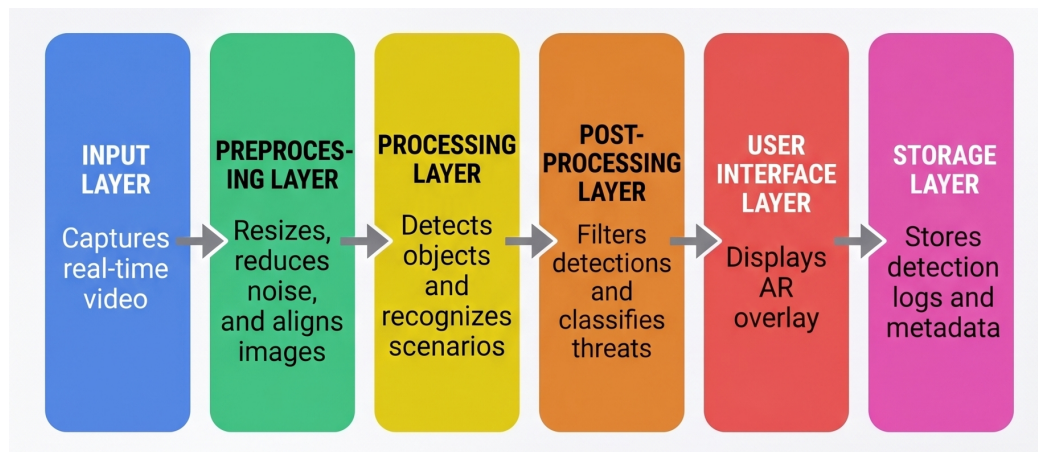
Figure 4.1: System Architecture
