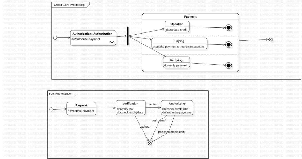
StateMachine1:StatechartDiagram1
