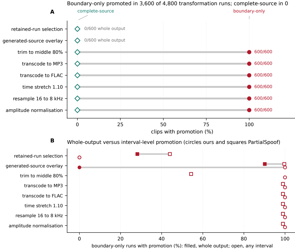
Figure 4: Promotion by transformation, 600 mixed-origin clips per transformation processed by stock FFmpeg, 4800 runs in all. (A) Whole-output claim: filled circle, boundary-only reference policy; open diamond, complete-source propagation. Boundary-only promoted in 3600 runs and complete-source in 0. (B) The same boundary-only runs scored per interval, on our corpus (circles) and on PartialSpooF (squares, Section 7.5); filled marks count whole-output promotion, open marks promotion in any interval. Overlay’s whole-output claim is correct while one of its intervals promotes. Complete-source propagation promoted in no interval on either corpus. The baseline is a constructed policy, and these are counts over frozen corpora, not prevalence estimates.
