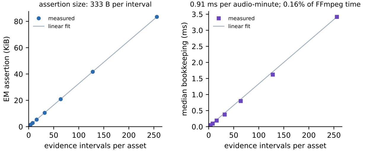
Figure 5: Cost of carrying interval evidence. The emitted assertion and the bookkeeping time both grow linearly in the number of evidence intervals, not in audio duration, so cost scales with how often ancestry changes along the timeline.
