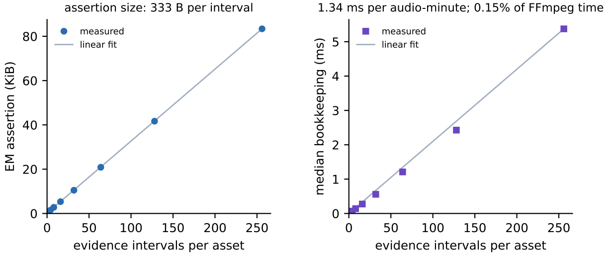
Figure 7: Cost of carrying interval evidence. The emitted assertion and the bookkeeping time both grow linearly in the number of evidence intervals, not in audio duration, so cost scales with how often ancestry changes along the timeline.
