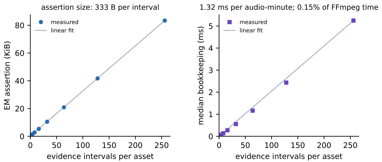
Figure 7: Cost of carrying interval evidence. The emitted assertion and the bookkeeping time both grow linearly in the number of evidence intervals, not in audio duration, so cost scales with how often ancestry changes along the timeline.
