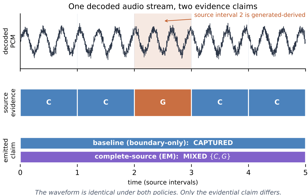
Figure 1: The minimal temporal counterexample. Five source intervals, of which the third is generated-derived. A boundary-only reading of the retained region sees captured evidence at both ends and may emit CAPTURED; the complete-source rule sees C + C + G + C + C and emits MIXED \{C, G\} . The decoded audio is identical under both policies.
