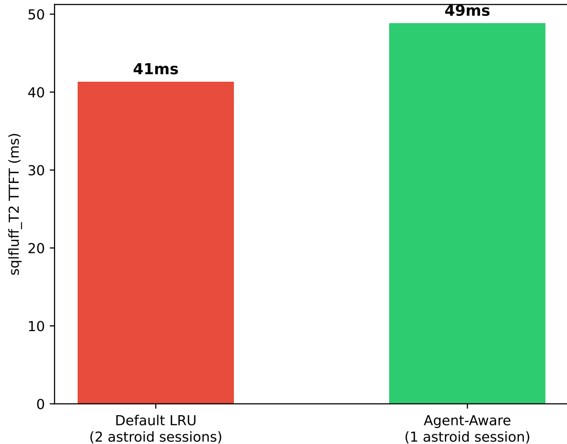
Recovery TTFT: LRU vs Agent-Aware [MEASURED]
