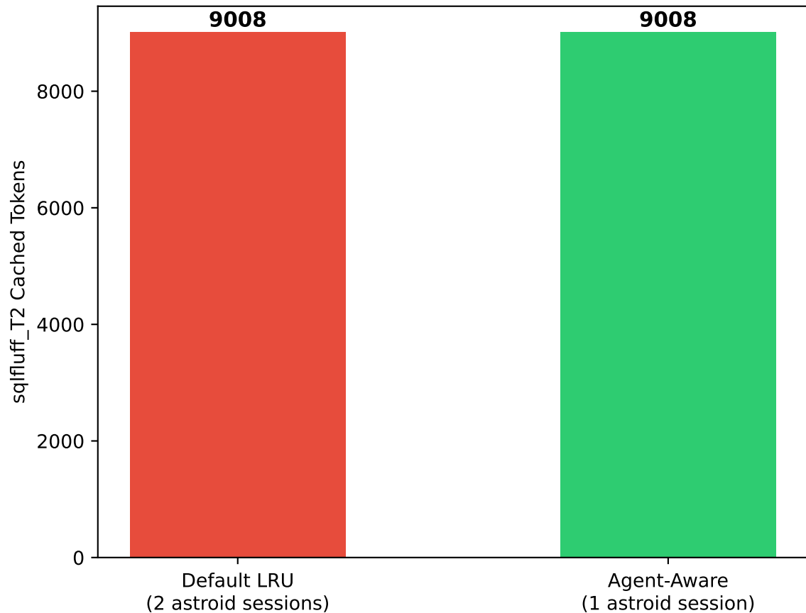
Prefix Survival: LRU vs Agent-Aware [MEASURED]
