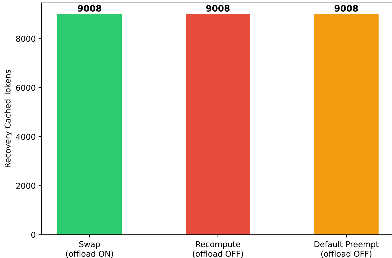
Prefix Cache Survival Under Different Preemption Strategies [MEASURED]
