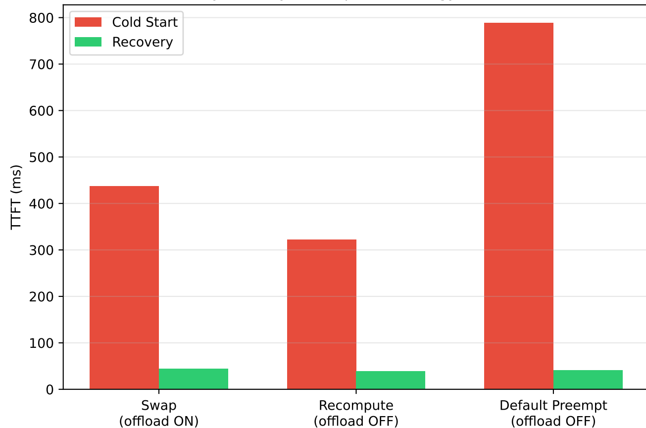
Recovery TTFT by Preemption Strategy [MEASURED]
