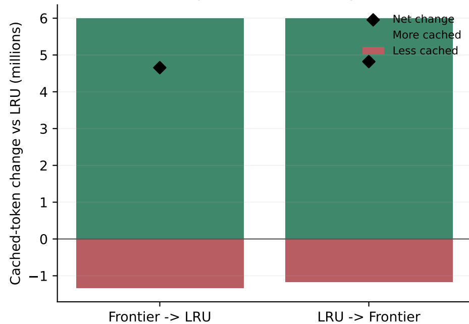
Whole-run gains include all regressions
