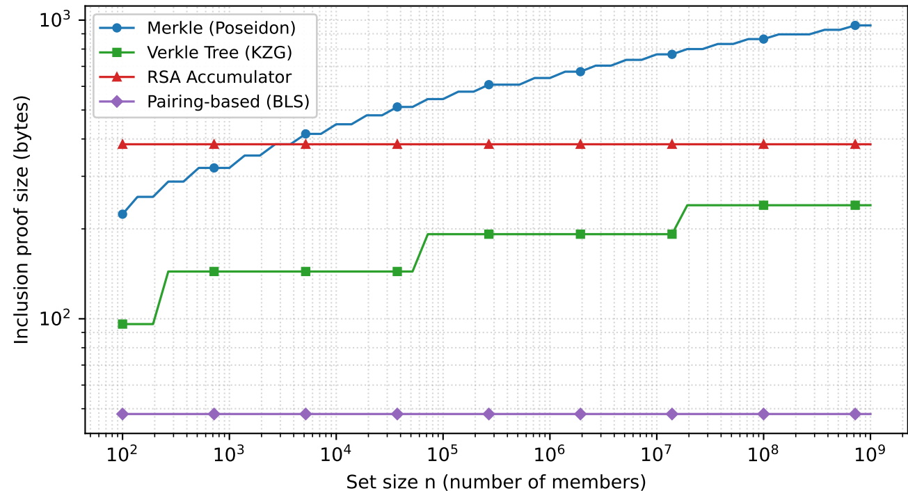
Inclusion Proof Size vs. Set Size, by Accumulator Type
