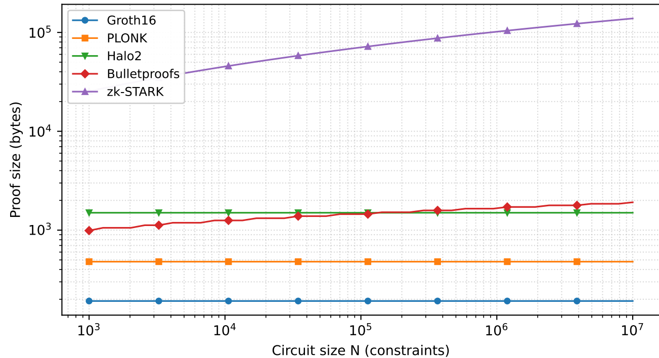
Proof Size vs. Circuit Size, by ZK Scheme
