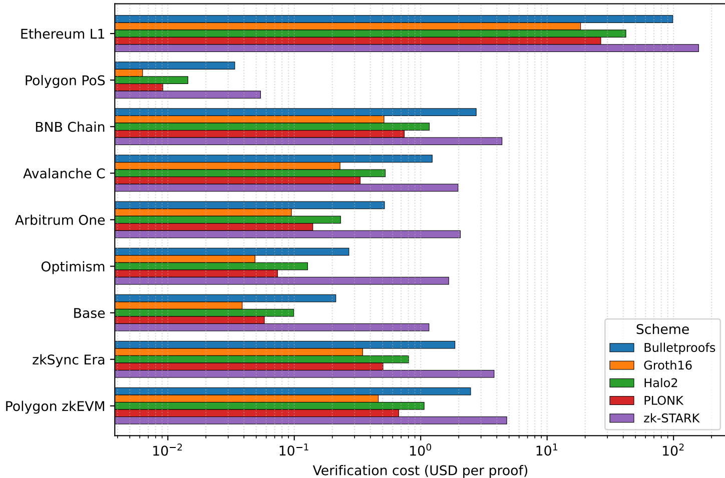
Cross-Chain Verification Cost by ZK Scheme
