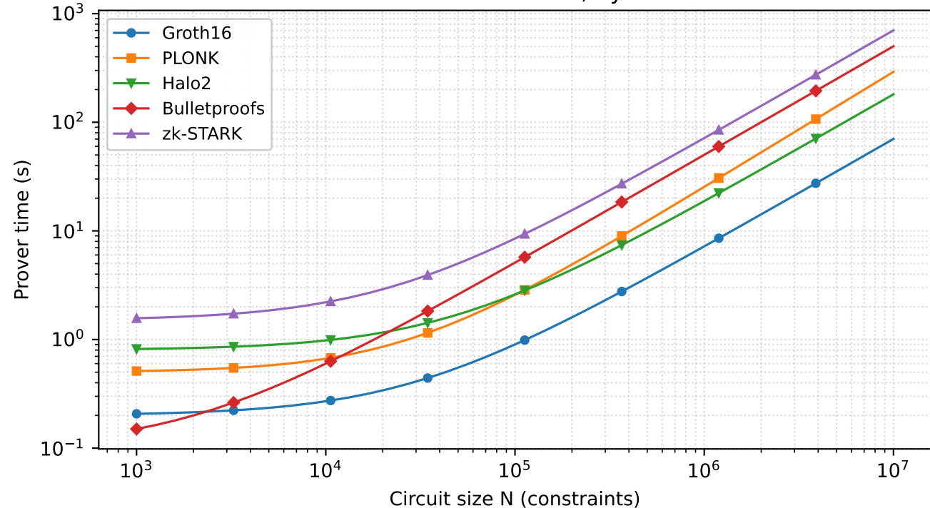
Prover Time vs. Circuit Size, by ZK Scheme
