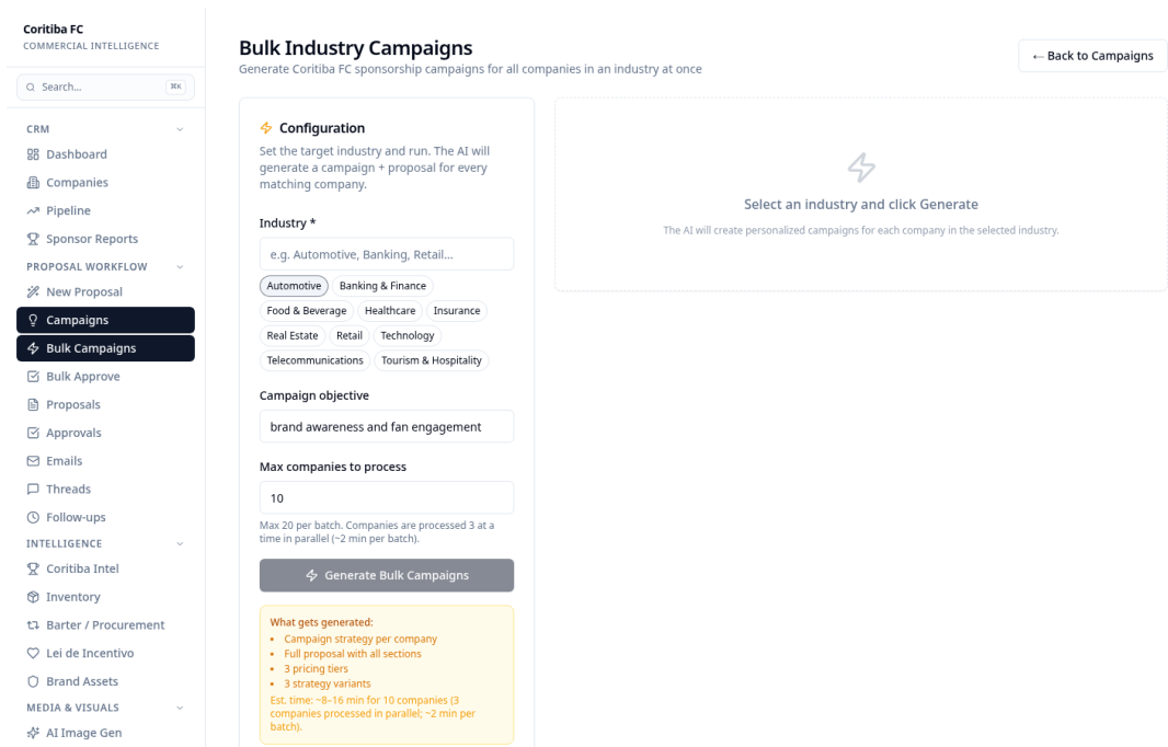
FR-01: Current Bulk Campaigns form
