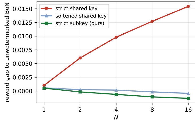
Selection shift (real model)
