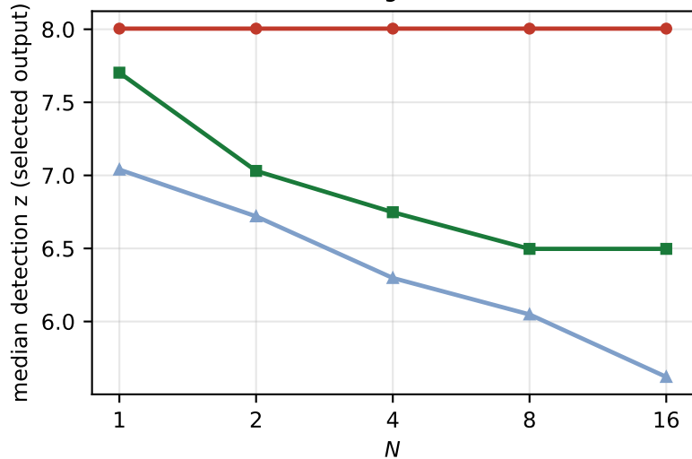
Watermark strength after selection
