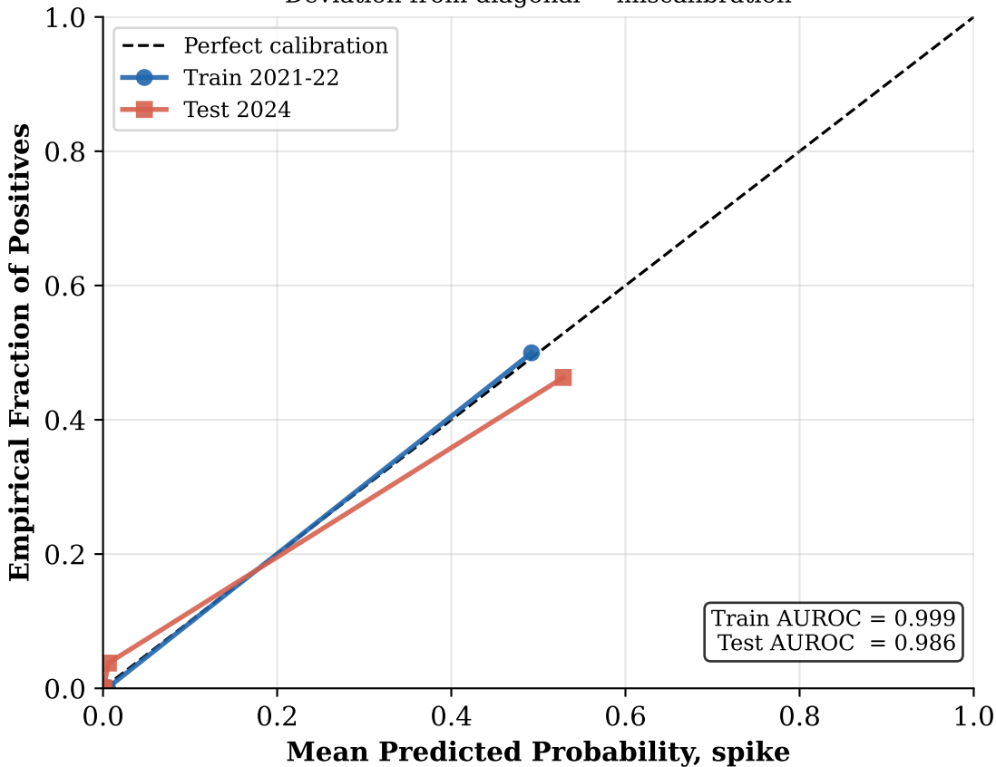
Figure 2: Classifier Calibration Curve Deviation from diagonal = miscalibration
