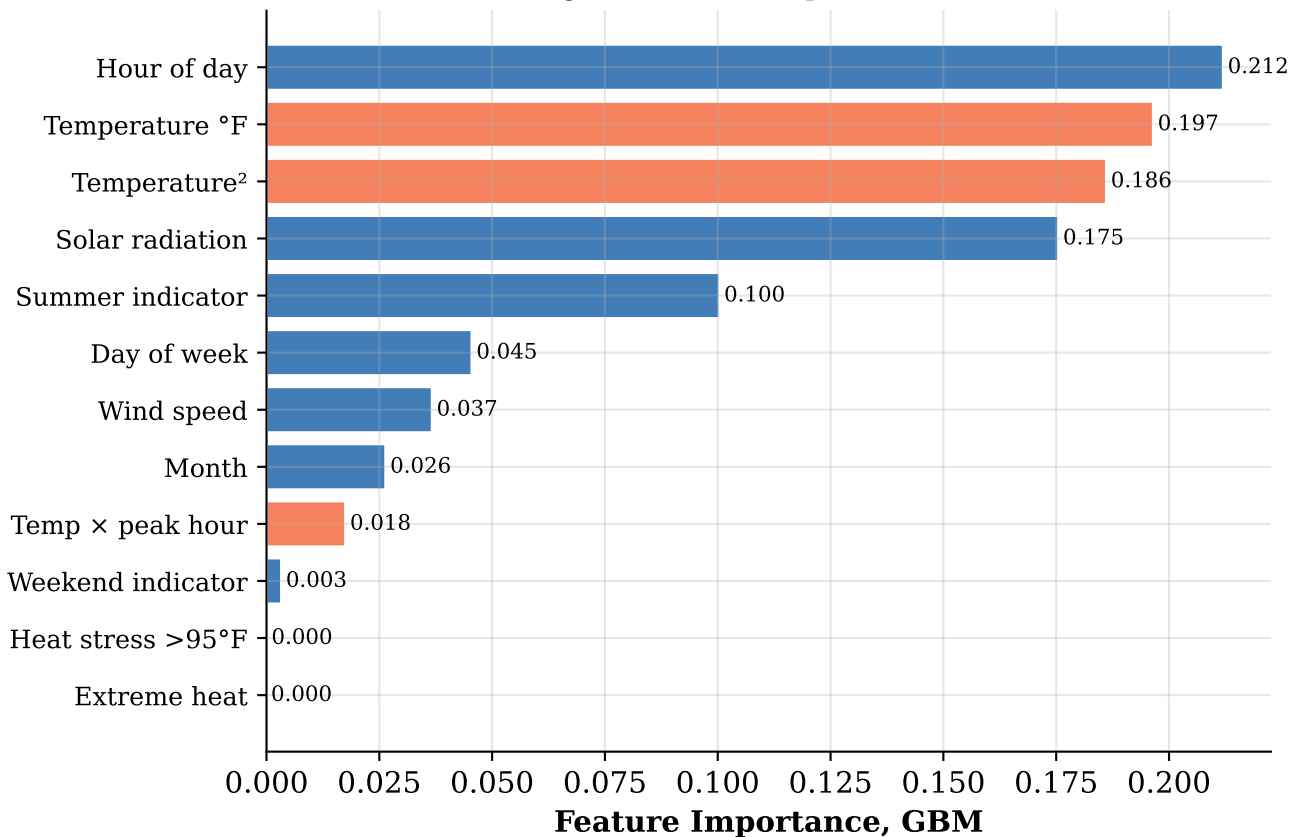
Figure 3: Feature Importances for Weather-Only Spike Classifier Orange = weather/temperature features
